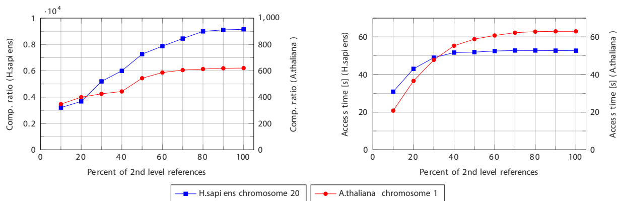
Figure 3. Influence of the percent of 2nd level references on GDC 2 compression ratio (left), decompression (access) time of a single sequence (right). In both cases the input dataset contained all available sequences.
