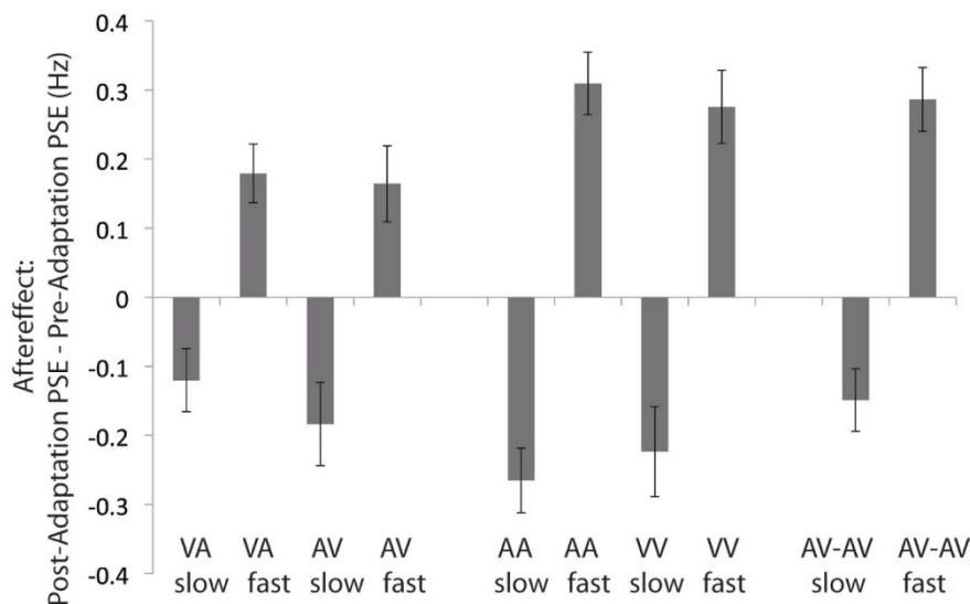
Figure 2 | Crossmodal, unimodal, and bimodal aftereffects. Participants ( N = 8 ) in the main experiment completed the rate classification task pre- and post-adaptation to relatively slow or fast stimuli for AV (auditory adaptor, visual test), VA (visual adaptor, auditory test), AA (auditory adaptor/test), VV (visual adaptor/test), and AV-AV (bimodal) conditions. The aftereffect was the post-adaptation PSE – pre-adaptation PSE. Error bars show 95% confidence intervals.
