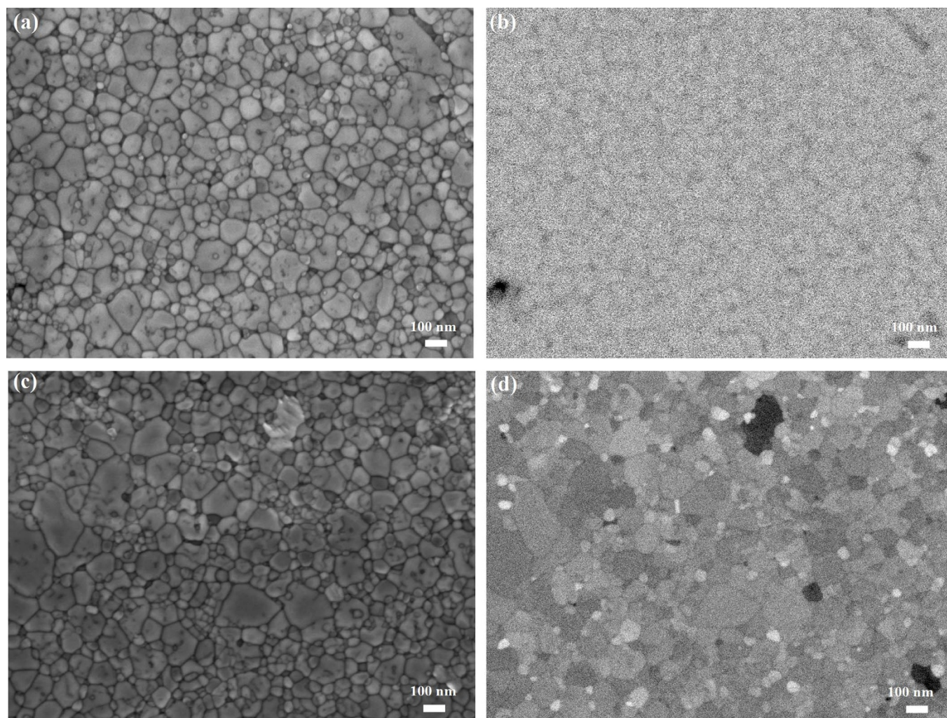
Figure 2 | High magnification SEM and BSE images of x = 0.08 (a–b), x = 0.12 (c–d). The Ce-rich area corresponds to brighter region and The Zn-rich area corresponds to darker region in (d).
