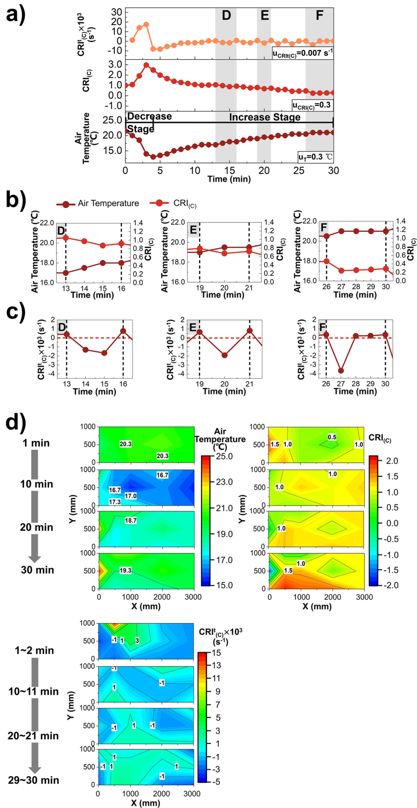
Fig. 3 CRI_{(C)}^t , CRI_{(C)} and Air Temperature. a The variation of CRI_{(C)}^t (reddish orange), CRI_{(C)} (red) and air temperature (deep red) at point (X,Y) = (500,1000) mm, whose uncertainty is u_{CRI_{(C)}^t} , u_{CRI_{(C)}} and u_T ( n = 151 samples). b The variation of air temperature (deep red) and CRI_{(C)} (red) during fluctuation cycle D( t = 13 - 16 \text{ min} ), E( t = 19 - 21 \text{ min} ), F( t = 26 - 30 \text{ min} ). c The variation of CRI_{(C)}^t (deep red) during fluctuation cycle D( t = 13 - 16 \text{ min} ), E( t = 19 - 21 \text{ min} ), F( t = 26 - 30 \text{ min} ). d The spatial distribution of air temperature and CRI_{(C)} at t = 1 \text{ min} , 10 \text{ min} , 20 \text{ min} and 30 \text{ min} , and CRI_{(C)}^t during t = 1\text{-}2 \text{ min} , 10\text{-}11 \text{ min} , 20\text{-}21 \text{ min} and 29\text{-}30 \text{ min} in the XOY plane ( X = 0\text{-}3000 \text{ mm} and Y = 0\text{-}1000 \text{ mm} ).
