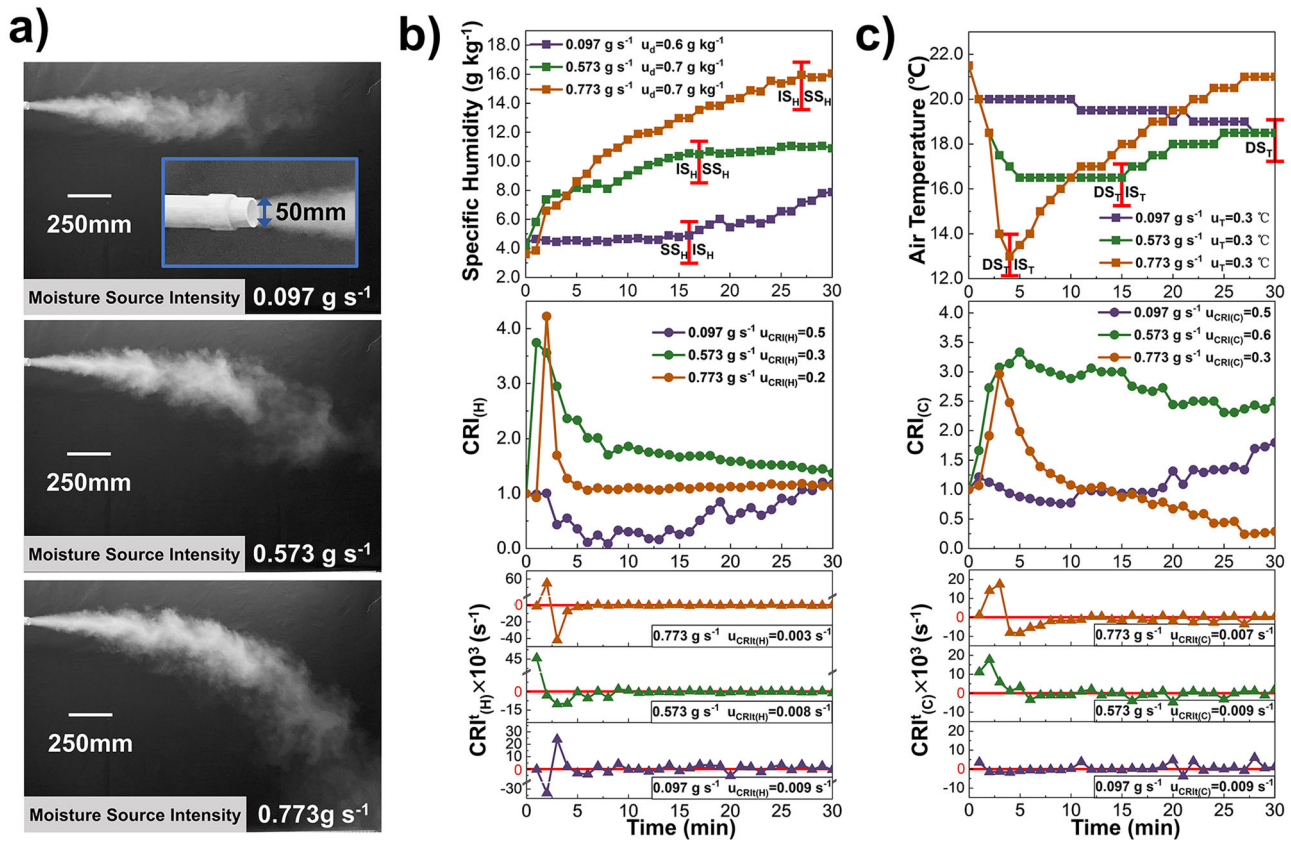
Fig. 5 Source Intensity. The variation of Air humidity and temperature, Contribution Ratio of Indoor Humidity ( \text{CRI}_{(H)} ) and Contribution Ratio of Indoor Climate ( \text{CRI}_{(C)} ), Rate of Humidity Contribution Change ( \text{CRI}_{(H)}^t ) and Rate of Indoor Climate Contribution Change ( \text{CRI}_{(C)}^t ) under conditions with various source intensities. a Moisture flows produced by the sources with intensities of 0.097 \text{ g s}^{-1} , 0.573 \text{ g s}^{-1} and 0.773 \text{ g s}^{-1} , respectively. b The variation of specific humidity (curves with squares), \text{CRI}_{(H)} (curves with dots) and \text{CRI}_{(H)}^t (curves with triangles) at point (X,Y) = (500,1000) mm influenced by the sources with intensities of 0.097 \text{ g s}^{-1} (purple), 0.573 \text{ g s}^{-1} (green) and 0.773 \text{ g s}^{-1} (orange), whose uncertainty is u_{d_i} , u_{\text{CRI}_{(H)}} and u_{\text{CRI}_{(H)}^t} ( n = 130 samples, 118 samples and 151 samples). c The variation of air temperature (curves with squares), \text{CRI}_{(C)} (curves with dots) and \text{CRI}_{(C)}^t (curves with triangles) at point (X,Y) = (500, 1000) mm influenced by the sources with intensities of 0.097 \text{ g s}^{-1} (purple), 0.573 \text{ g s}^{-1} (green) and 0.773 \text{ g s}^{-1} (orange), whose uncertainty is u_T , u_{\text{CRI}_{(C)}} and u_{\text{CRI}_{(C)}^t} ( n = 130 samples, 118 samples and 151 samples).
