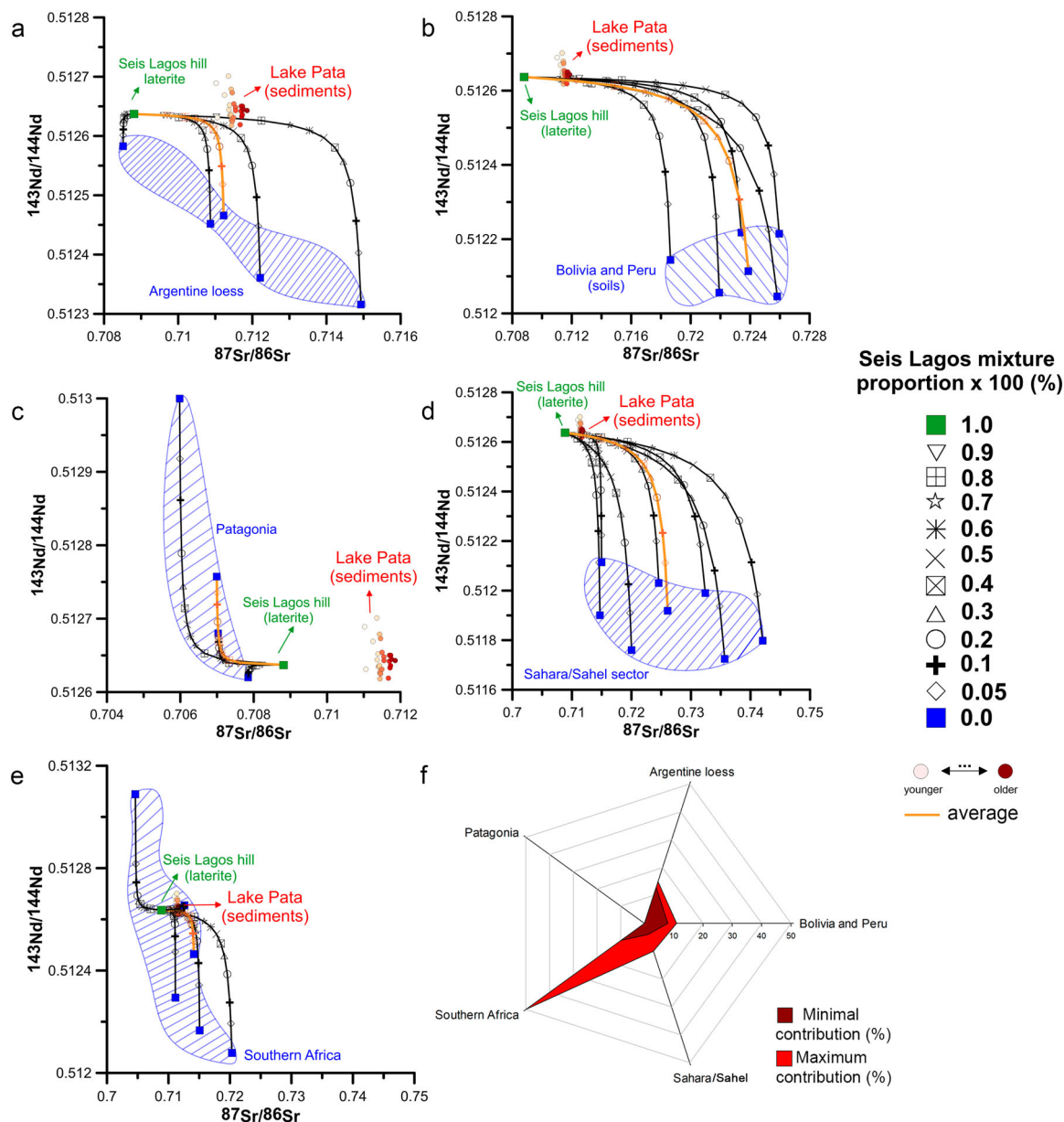
Fig. 5 Binary mixing curves 56 between the Seis Lagos hill lateritic crust, where Lake Pata is inserted, and the different possible dust sources.
