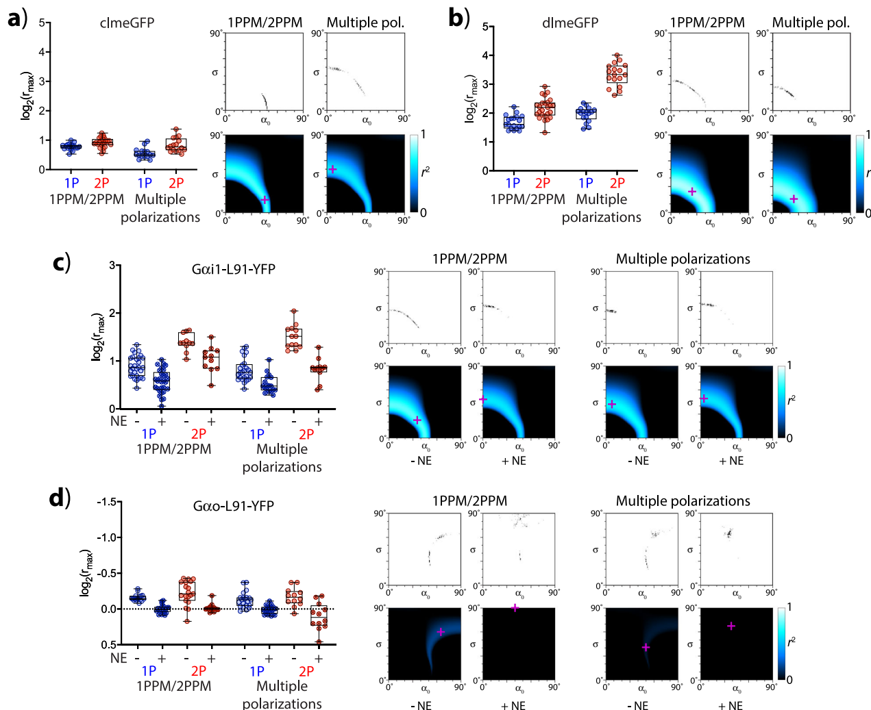
Fig. 8 Quantitative polarization microscopy imaging of intact, living cells. a Cells expressing the model lipidated fluorescent protein construct clmeGFP . Left: a plot of \log_2(r_{\max}) values obtained from 1PPM, 2PPM, and from multiple polarization measurements using 1P and 2P excitation, with median values, 25 th and 75 th percentiles, and ranges shown; Right: plots showing combinations of \alpha_0, \sigma consistent with combined 1PPM/2PPM, and 1P/2P multiple-excitation polarization observations (top: 95% confidence interval estimates obtained by bootstrapping, bottom: heat-maps of goodness of fit, described by the coefficient of determination r^2 ). The \alpha_0, \sigma combination in best agreement with microscopy data is indicated by a magenta cross. b Same as a , but for dlmeGFP . c Same as (a) and (b) , but for Gαi1-L91-eYFP , before and after activation by norepinephrine (NE). d Same as (c) , but for Gαo-L91-eYFP .
