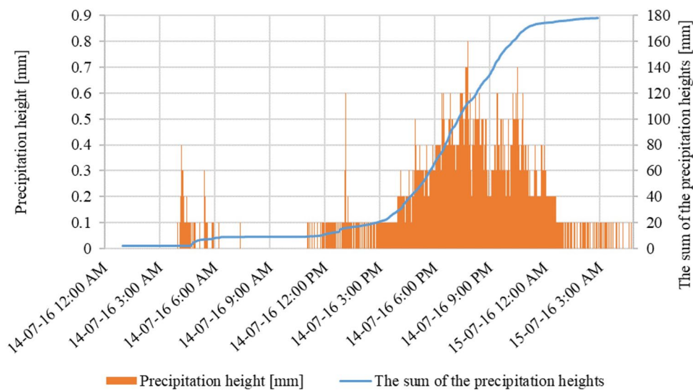
Figure 9. Total precipitation curve, measured in Gdańsk Oliwa on July 14–15th, 2016.
