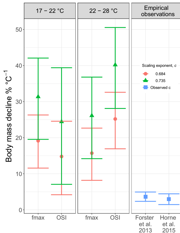
Figure 1. Predicted and observed declines in body mass of aquatic ectotherms with increasing temperature (temperature-size rule slopes, error bars \pm 95\% CI). “ fmax ” gives the predicted slopes based on empirical measurements of fmax , and “ OSI ” those based on the oxygen supply index. Slopes were estimated for two temperature intervals, and for the two boundary values of the surface area-body mass scaling exponent c (red circles c = 0.684, green triangles c = 0.735). Values (mean \pm 1.96 SE) from two meta-analyses of aquatic ectotherms are given for comparison.
