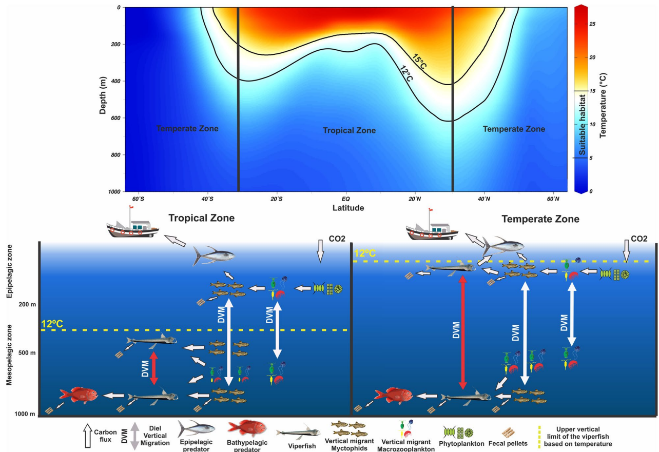
Figure 7. Conceptual model exhibiting global suitable vertical habitat of the viperfish Chaulichodus sloani based on temperature profiles (Source: Word Ocean Atlas 73 ) and differences in the vertical migration and trophic interactions of this species in the tropical and temperate waters. Temperature information from the upper panel refers to the meridional Sect. 30°.
