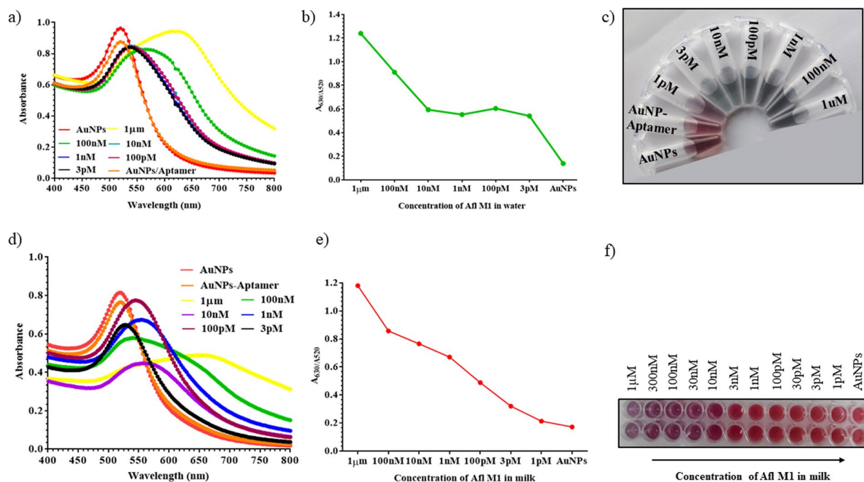
Figure 3. (a) UV-Vis spectra of aptamer modified AuNPs with different concentrations of Aflatoxin M1 in water (1 \mu M to 1 pM) and (b) Absorbance peak ratio at A_{630/520} nm; (c) Image of different concentrations of Aflatoxin M1 in water; (d) UV-Vis absorption spectra of aptamer modified AuNPs with different concentrations of Aflatoxin M1 spiked in milk (1 \mu M to 1 pM) and (e) Absorbance peak ratio of A_{630/520} nm; (f) Image of different concentrations of Aflatoxin M1 with aptamer modified AuNPs.
