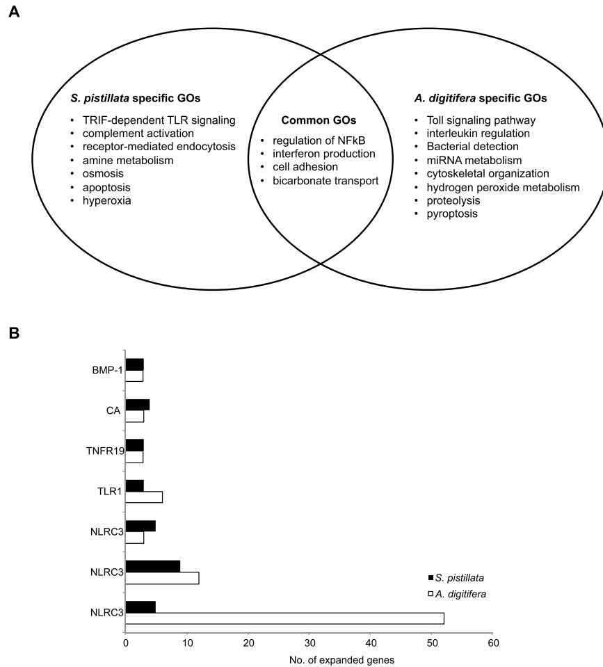
Figure 3. Overview of processes and proteins associated with gene expansions in S. pistillata and A. digitifera . (A) Gene Ontology (GO) enrichment of Biological Process (BP) category ( p < 0.05 ) of many-to-one and many-to-many orthologs for S. pistillata and A. digitifera (Dataset S5). (B) Ortholog groups with independently expanded genes in both coral species show different degrees of expansions in both corals and featured many immunity-related genes (Dataset S6). Notably, the NLRC3 examples belong to three distinct ortholog groups (Dataset S6). BMP-1 = Bone Morphogenetic Protein 1; CA = Carbonic Anhydrase; TNFR19 = Tumor necrosis factor receptor superfamily member 19; TLR1 = Toll-like receptor 1; NLRC3 = NOD-like receptor C3.
