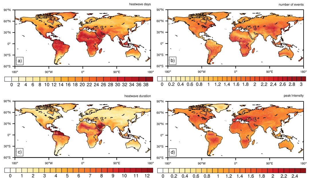
Figure 1. Median regression coefficients estimated from the CMIP5 model ensemble between global warming ( ^{\circ}\text{C} ) and seasonal (a) heatwave days; (b) number of events; (c) event duration; and (d) peak heatwave intensity. Created using NCAR Command Language (version 6.4.0) [Software]. (2017). http://dx.doi.org/10.5605/D6WD3XH5 .
