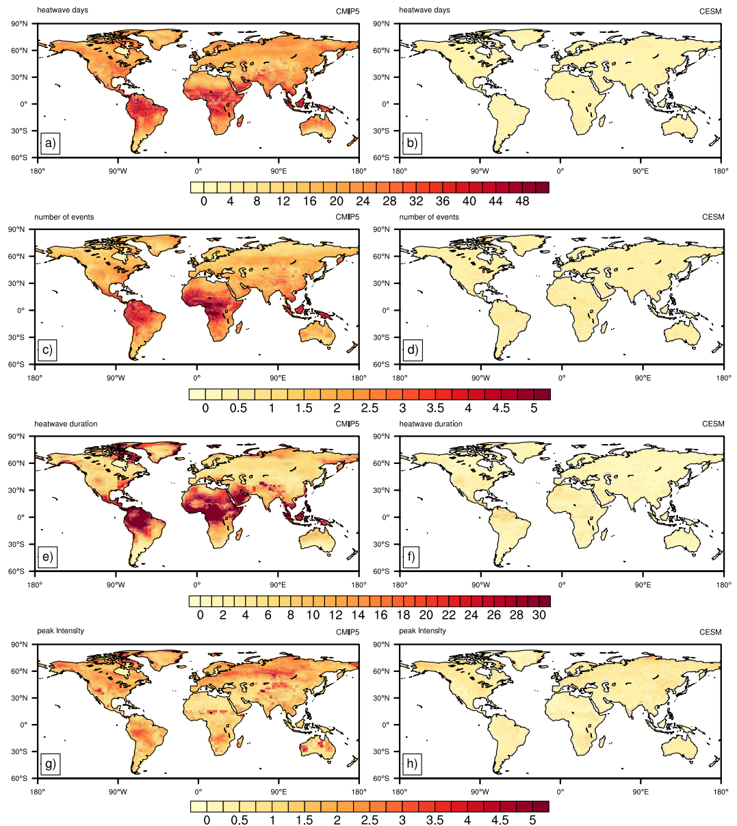
Figure 3. Spread in the regression coefficient estimated from CMIP5 models (left column) and the CESM ensemble (right column) for (a,b) heatwave days; (c,d) number of events; (e,f) event duration; and (g,h) peak intensity. The spread is given by the ensemble 1 st percentile subtracted from the ensemble 99 th percentile. Created using NCAR Command Language (version 6.4.0) [Software]. (2017). http://dx.doi.org/10.5605/D6WD3XH5 .
