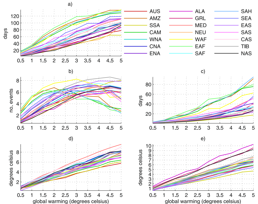
Figure 2. Regional (see Giorgi and Francisco, 2000) changes in heatwaves relative to 0.5°C global warming thresholds estimated from the median of the CMIP5 model ensemble for (a) heatwave days; (b) number of events; (c) event duration; (d) peak intensity; and (e) regional mean warming. See table S.2 for region boundaries.
