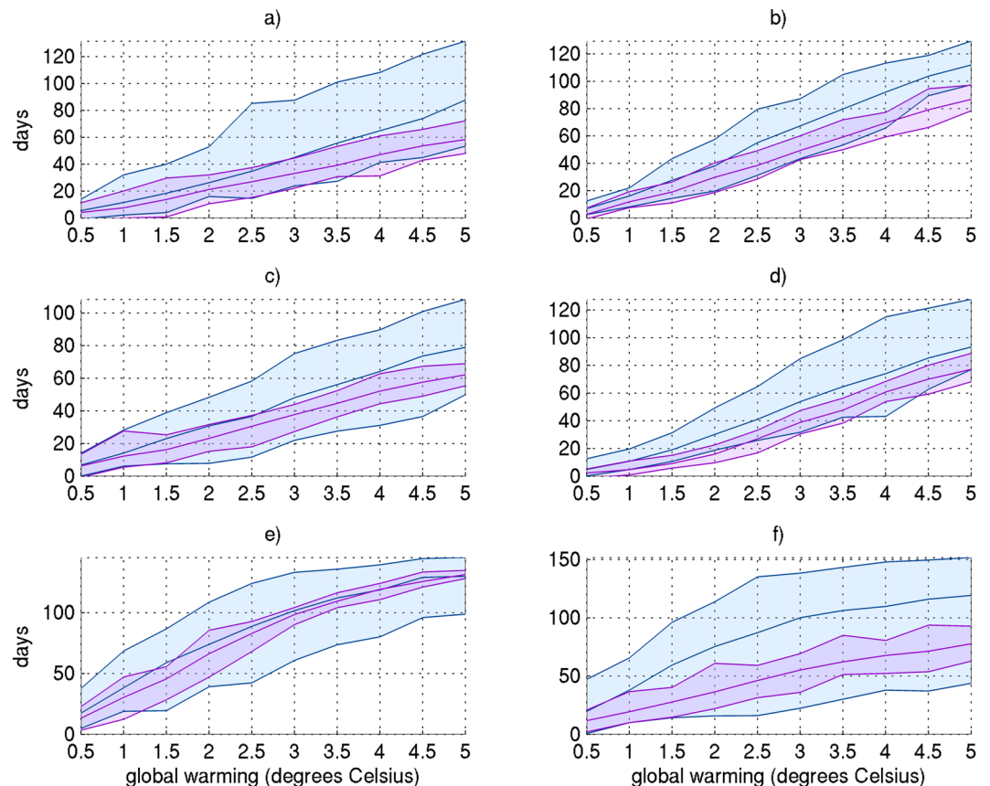
Figure 4. Ensemble spread (99 th percentile – 1 st percentile) of increases in the number of heatwave projected by the CMIP5 ensemble (blue) and CESM ensemble (purple) per 0.5°C global warming, for (a) Alaska; (b) the Mediterranean; (c) Australia; (d) East Asia; (e) the Amazon, and (f) East Africa. These regions were chosen as they are representative of all 21 regions analysed. Note that the spread due to internal variability (estimated from CESM) is reasonably consistent across the thresholds. See table S.2 for region boundaries.
