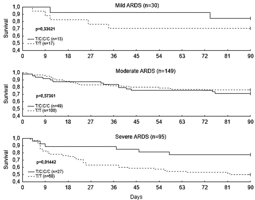
Figure 1. Kaplan-Meier survival analysis. Kaplan-Meier survival analysis of 90-day survival according to FER rs4957796 for the three acute respiratory distress syndrome (ARDS) groups. FER polymorphism rs4957796 is associated with higher 90-day mortality exclusively in patients with severe ARDS due to pneumonia ( p = 0.0144 , log-rank test).
