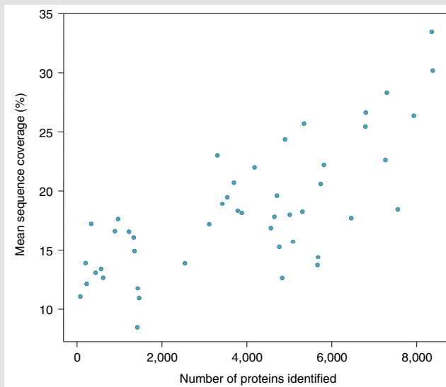
Sequence coverage in global proteomics studies. MS-based global proteomics studies identify and quantify proteins with variable sequence coverage. The single best run from the 47 publications present in ProteomicsDB shows how sample-specific protein sequence coverage improves with sample preparation methods. Sequence coverage generally decreases with sample complexity and increases with time (cost) dedicated to studying the sample.
