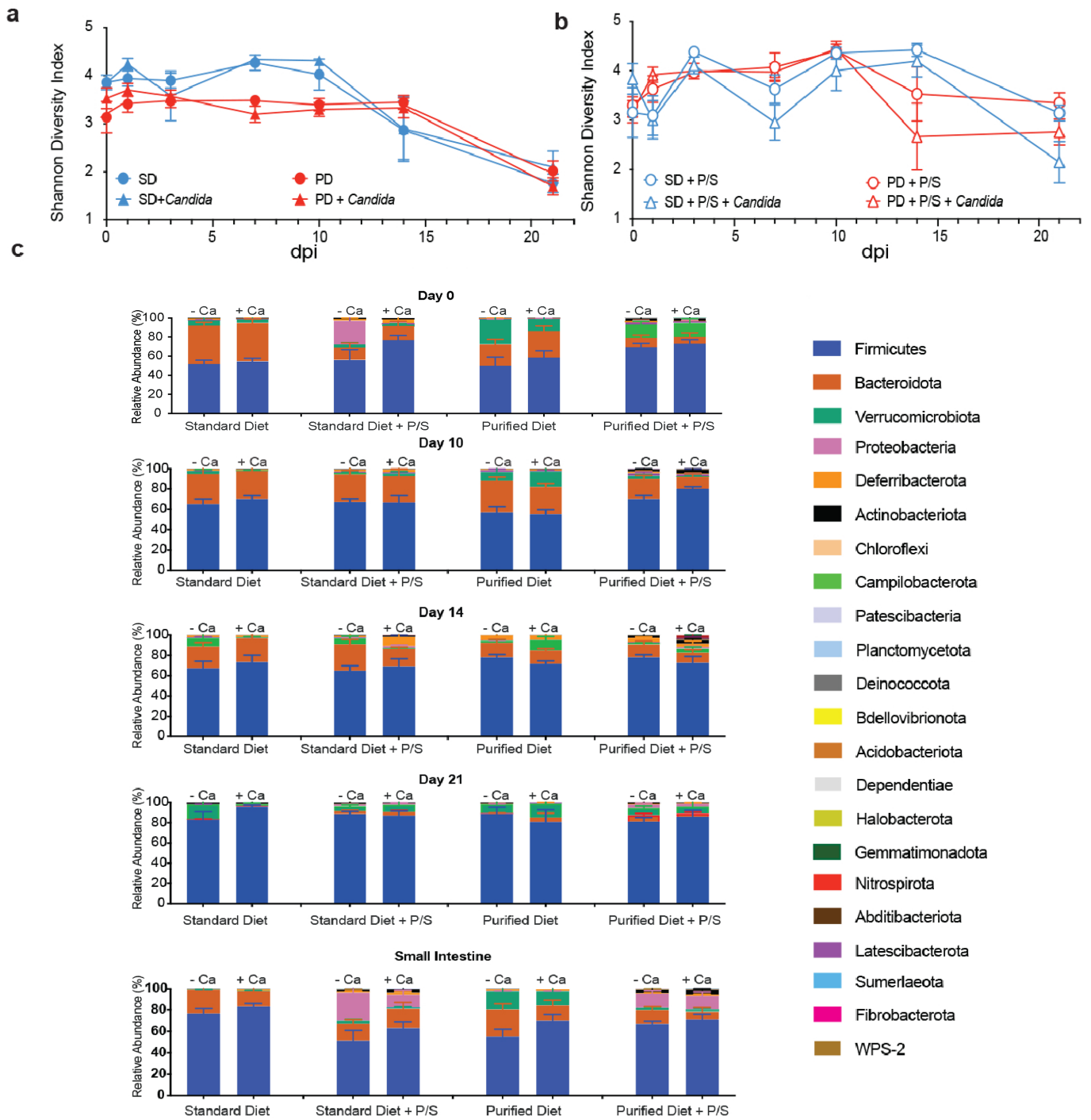
Extended Data Fig. 5 | Analysis of gut bacterial populations in different murine models. 16S rRNA sequencing data was used to determine the relative abundance of bacterial phyla in BALB/c colonization experiments using mice fed the SD or PD, and supplemented or not supplemented with antibiotics (P/S; penicillin/streptomycin). Each group of mice were also compared +/- inoculation
