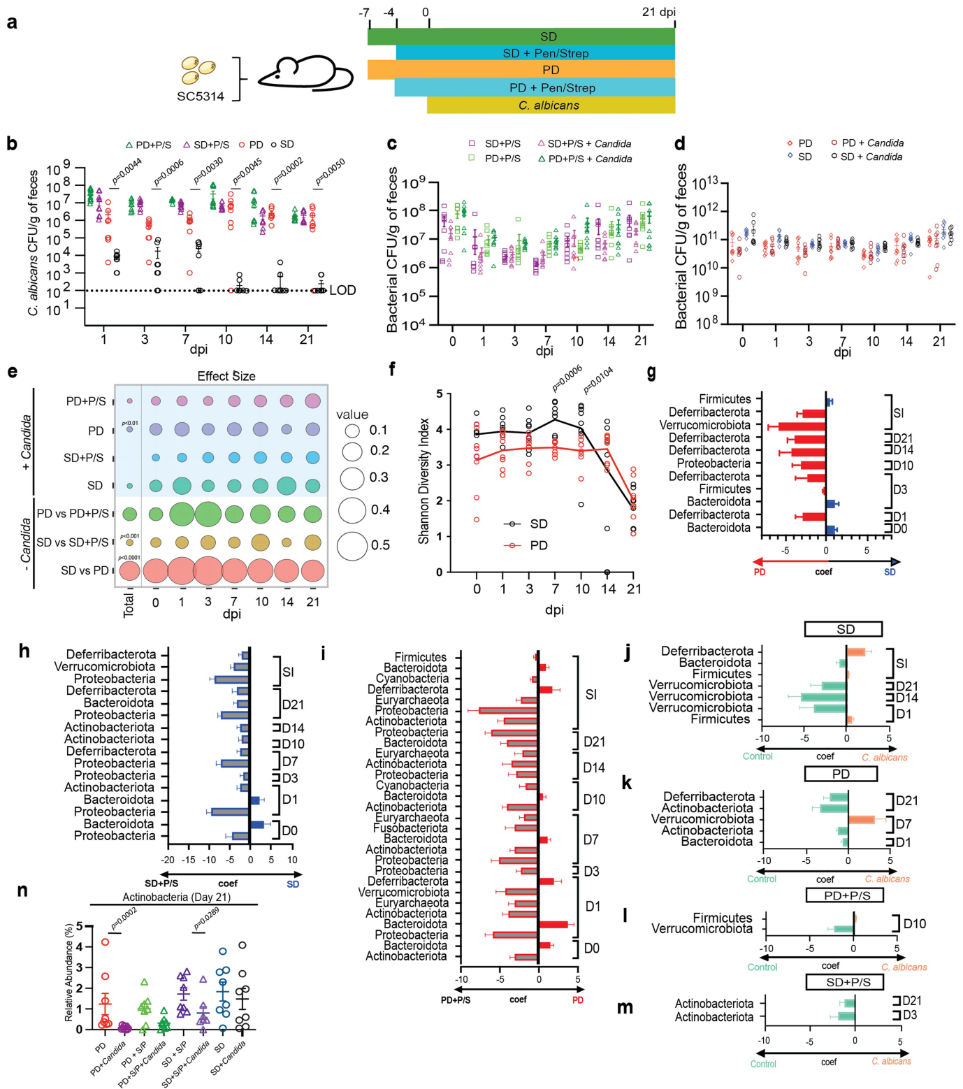
Extended Data Fig. 3 | Analysis of microbiome composition upon changes in diet, antibiotic treatment, and C. albicans colonization. a , Schematic of colonization experiments. BALB/c mice were fed the SD or PD, with or without antibiotics (P/S; penicillin/streptomycin). These groups were compared with and without colonization with C. albicans SC5314 cells. b , C. albicans CFUs in fecal pellets collected at the indicated time points. LOD, limit of detection. n = 8 . c, d , Total bacterial levels in fecal pellets collected at the indicated time points by quantitative PCR in SD- or PD-fed mice with antibiotics ( c ) and without antibiotics ( d ). n = 8 . e , Bubble plot depicting the amount of variation in gut microbial composition determined by Permutational Multivariate Analysis of Variance (PERMANOVA) analysis using the adonis function and
