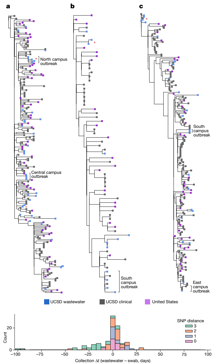
Fig. 6 | Wastewater identifies clinically known and unknown virus transmission. a–c , Maximum likelihood phylogenetic trees for each of the dominant VOCs (Epsilon ( a ), Alpha ( b ) and Delta ( c )) using high-quality samples obtained at UCSD, as well as a representative set of sequences from the entire United States. Wastewater sequences from the same sampler that differ by one or fewer SNPs are denoted with a red asterisk. For all sequences, consensus bases were called at sites with more than 50% nucleotide frequency. Location information is provided for select outbreaks. d , Pairwise comparison of collection date for matching and near-matching wastewater and nasal swab samples obtained at UCSD. Positive values indicate earlier collection in nasal swabs and negative values indicate earlier detection in wastewater.
