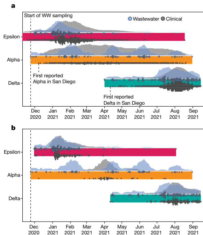
Fig. 3 | Freyja recovers early and cryptic transmission of SARS-CoV-2 variants of concern. a , Timeline and normalized epidemiological curves for VOC detection in both wastewater and clinical sequences from San Diego County (includes wastewater samples collected from Point Loma wastewater treatment plant, UCSD, as well as public schools in the San Diego districts) for the three major VOCs in circulation during the sampling period ( n = 475 wastewater, n = 22,504 clinical). Both Alpha and Delta variants are detected first in wastewater before clinical samples. Markers for clinical detections correspond to the ceiling of the daily detection count divided by 30 (for example, 1–30 samples = one marker, 31–60 = two markers), whereas wastewater markers correspond to a single detection. b , Timeline and epidemiological curves for VOC detection in the campus samples ( n = 364 wastewater, n = 333 clinical). Markers correspond to a single detection event for both clinical and wastewater surveillance. All wastewater detections correspond to an estimated VOC prevalence of at least 10%.
