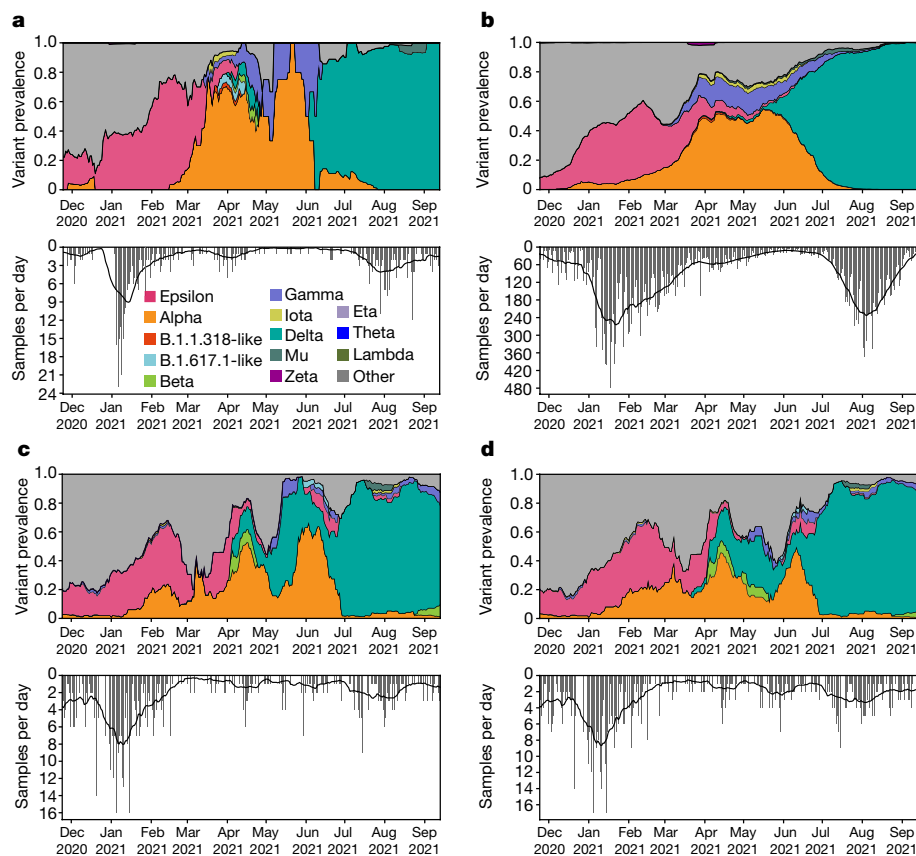
Fig. 4 | Deconvolution recovers a fine-grained estimate of virus population dynamics. a, b , Prevalence of SARS-CoV-2 variants in UCSD clinical surveillance ( a ) and variant prevalence in all clinical samples collected in San Diego County ( b ). c, d , Variant prevalence in wastewater at UCSD ( c ) and the greater San Diego
