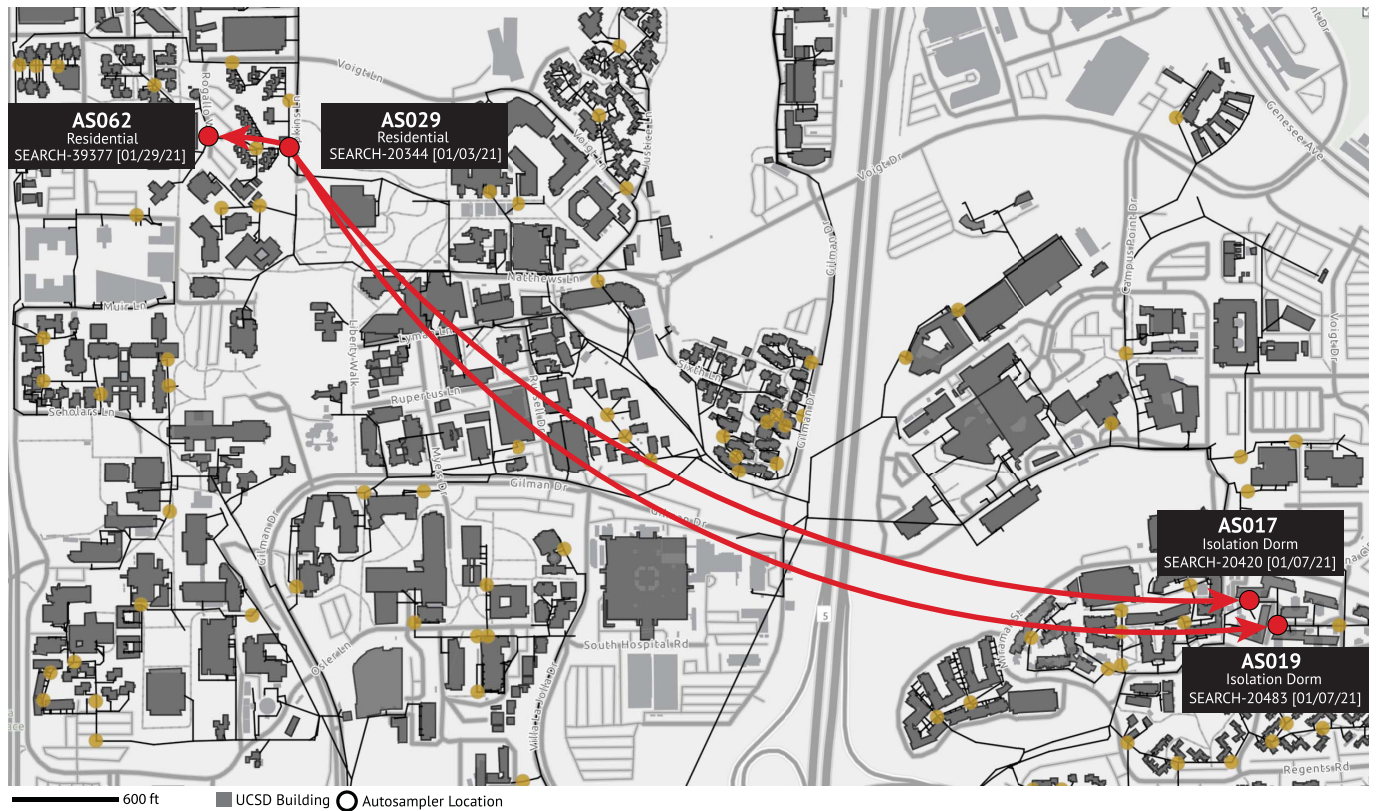
Extended Data Fig. 7 | Temporal and spatial dynamics of an Epsilon outbreak at UCSD. After initial detection on January 3rd 2021, infected individuals were transferred to isolation housing where they continued to shed virus. At the end of January, a matching virus was detected in a residence nearby
