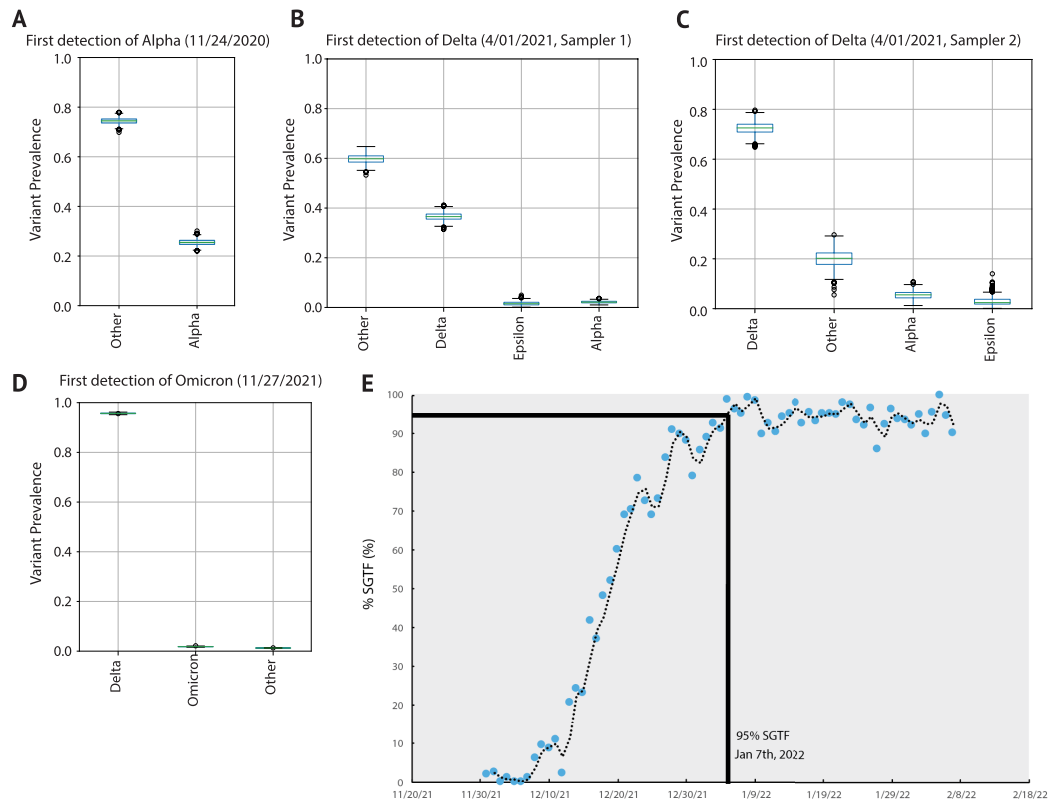
Extended Data Fig. 6 | Quantification of deconvolution uncertainty in first detection of VOCs. A-D. Bootstrap distributions of Freyja abundance estimates obtained by resampling read data from each sample corresponding to the first detection of that VOC in San Diego 1000 times with replacement. In all boxplots, box edges specify the first and third quartiles, solid line indicates the median, and whiskers delimit the maximum and minimum values within 1.5 times the inter-quartile range (IQR) of box edges. Outliers are denoted with individual markers. Two samplers were found to contain Delta on the same day. First detections were also confirmed using a VOC qPCR panel, as shown in Fig. 2
