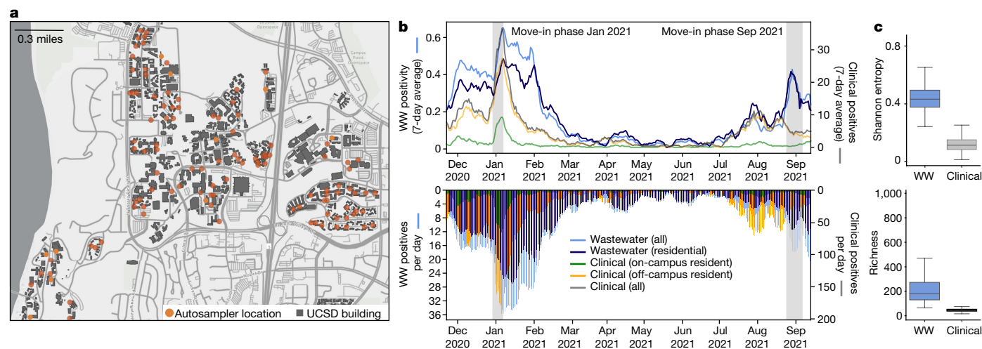
Fig. 1 | Campus sampling locations and SARS-CoV-2 testing statistics. a , Geospatial distribution of the 131 actively deployed wastewater autosamplers and the corresponding 360 university buildings on the campus sewer network. Building-specific data have been de-identified in accordance with university reporting policies. b , Campus wastewater (WW) and diagnostic testing statistics over the 295-day sampling period (positivity is the fraction of WW samplers with a positive qPCR signal). c , Virus diversity in wastewater and
