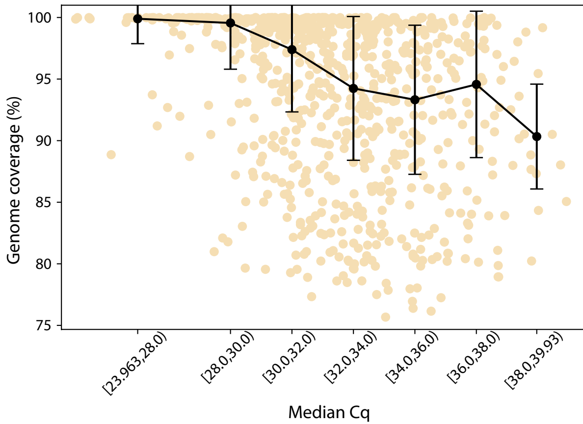
Extended Data Fig. 2 | Relationship between genome coverage and cycle quantification values. 10x genome coverage (fraction of sites with 10 reads or greater) remains high, even for Cq values of nearly 38 (n = 786). Points indicate median value in each bin, while error bars indicate the median absolute deviation.
