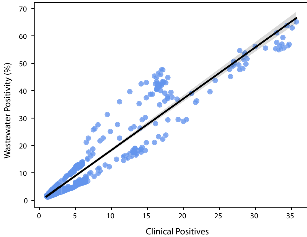
Extended Data Fig. 1 | Relationship of daily UCSD campus wastewater sampler positivity and campus clinical positives. Black line indicates the linear regression fit (slope = 1.88%/clinical positive, intercept = -0.45%) to the
