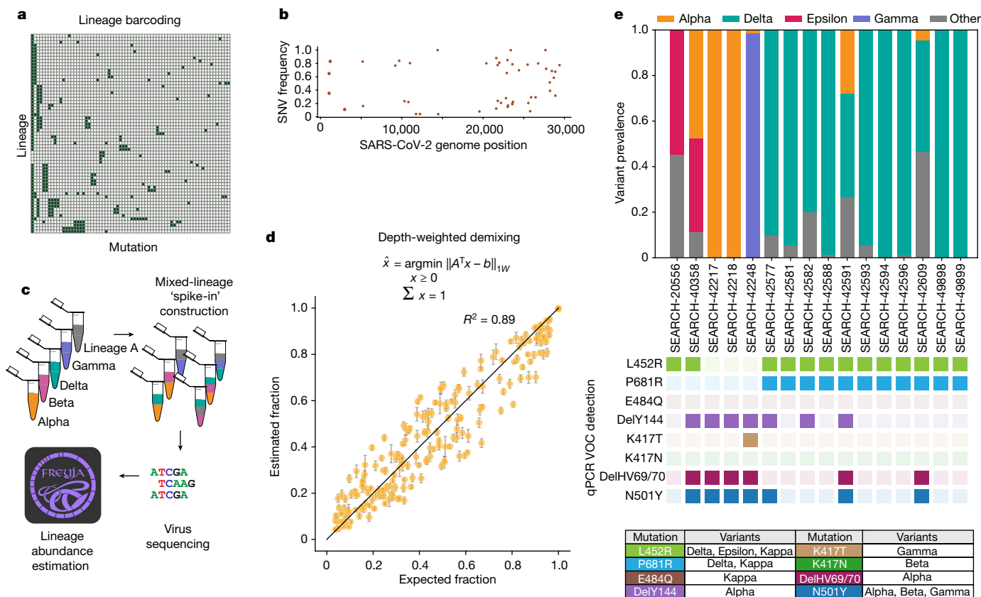
Fig. 2 | Sample deconvolution robustly recovers relative virus abundance.
