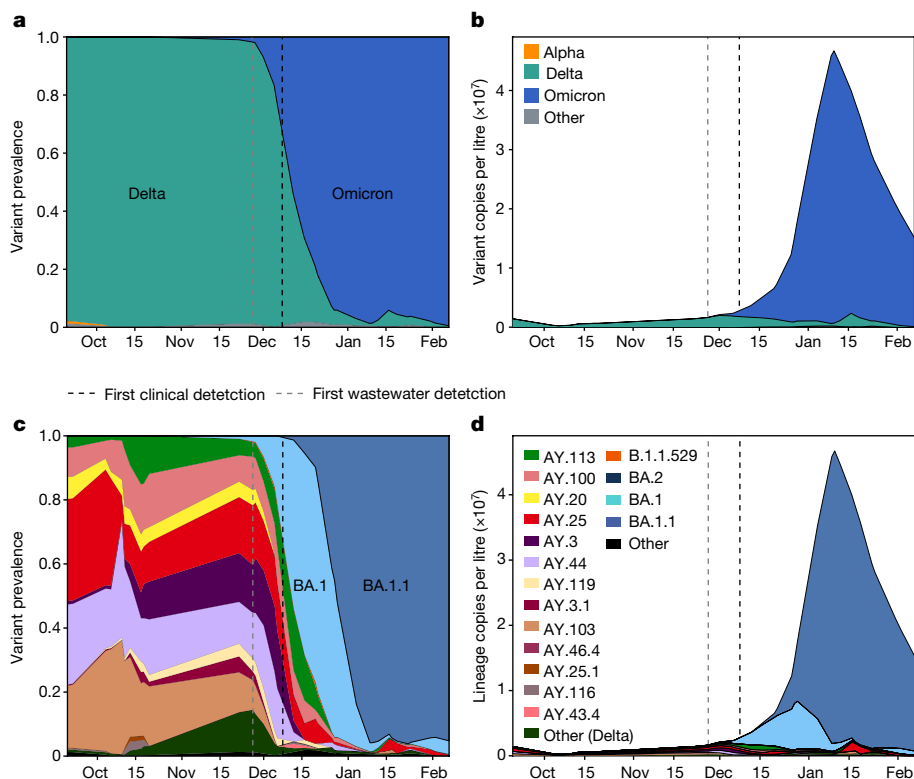
Fig. 5 | Community wastewater enables early Omicron detection and reveals lineage dynamics. a , Prevalence of SARS-CoV-2 VOCs in wastewater collected from the Point Loma wastewater treatment plant from late September 2021 to early February 2022. b , Estimated VOC concentrations; prevalence estimates
