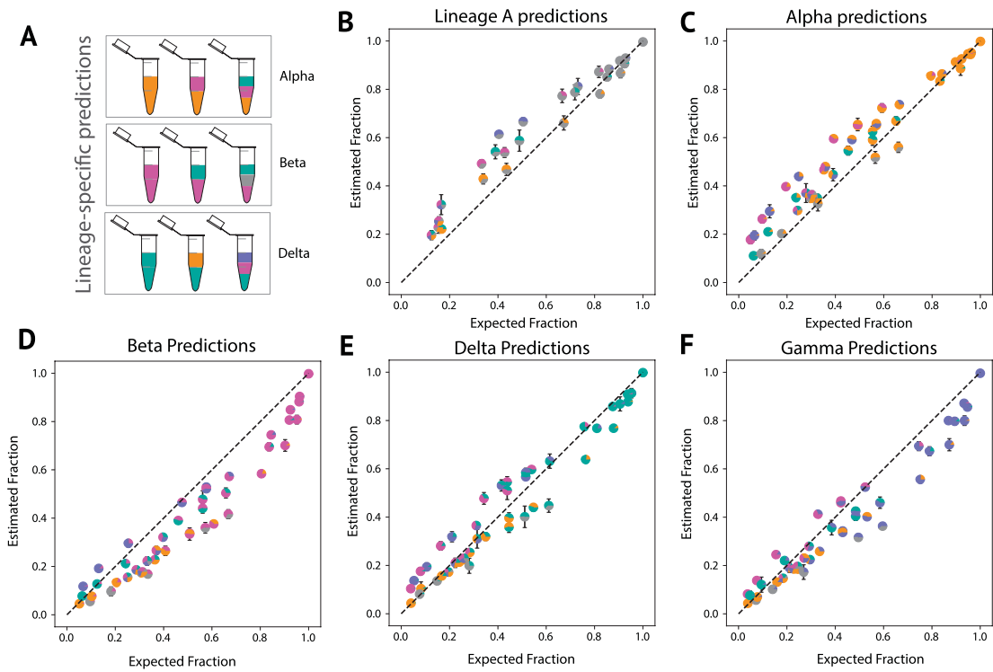
Extended Data Fig. 3 | Lineage-specific prediction of variant abundance in spike-in validation samples. A. Schematic of "spike-in" sample design. B-F. Lineage specific prediction. Proportions of each lineage in the sample are shown
