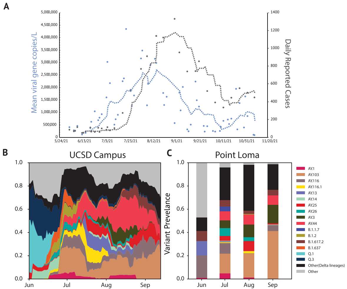
Extended Data Fig. 5 | The rise of the Delta variant during Summer 2021.
