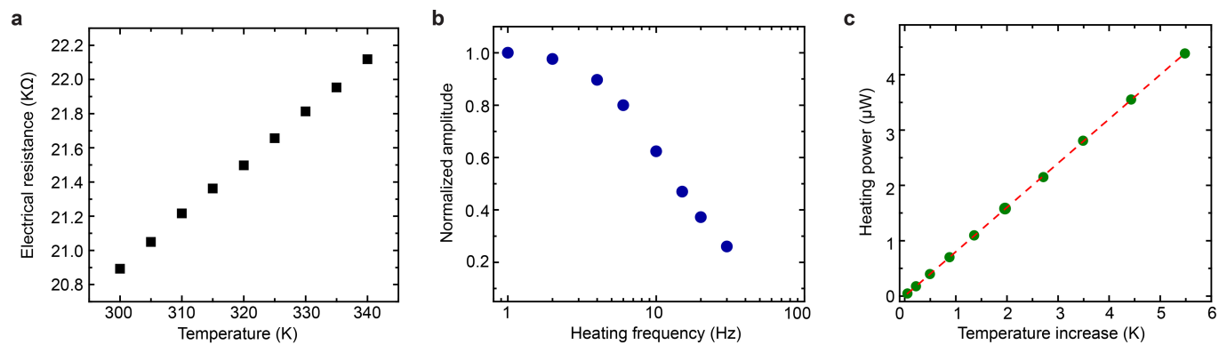
Extended Data Fig. 2 | Characterization of thermal and electrical properties of the scanning thermal probes. a, Measured electrical resistance of the Pt heater-thermometer as a function of temperature. b, Measured thermal response of the scanning probe as a function of the
