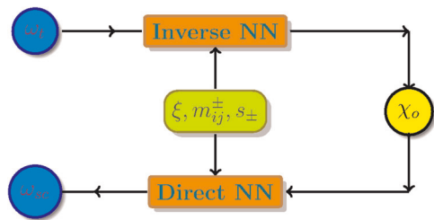
Fig. 16 Strategy to solve the inverse design problem for photonic devices, 325 where \chi_o is the structure parameter suggested by the inverse network and \xi , m_{ij}^{\pm} , and s_{\pm} are extra inputs for both networks. (Reprinted with permission from ref. 325 licensed under the CC BY 4.0 cc license.)
