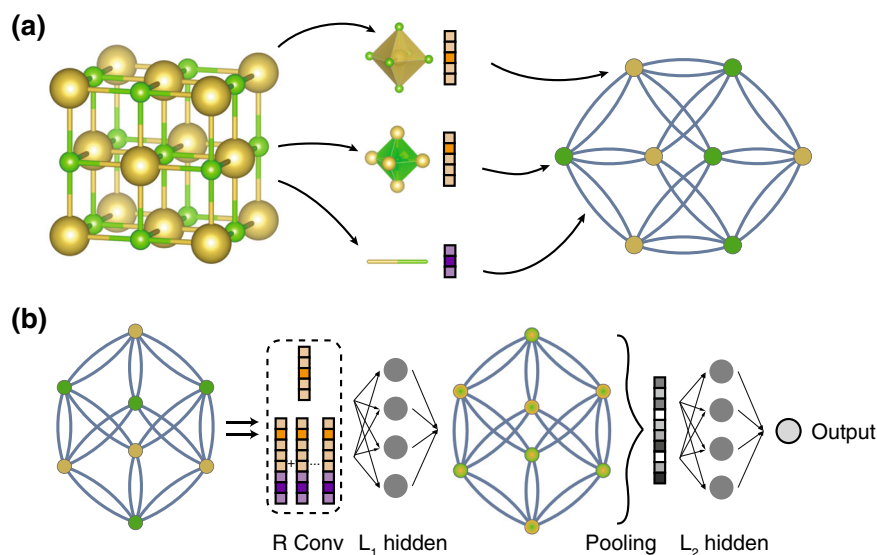
Fig. 6 Illustration of the crystal graph convolutional neural network. a Construction of the graph. b Structure of the convolutional neural network. (Reprinted with permission from ref. 40 . Copyright 2018 American Physical Society.)
