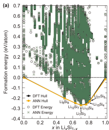
Fig. 18 Phase diagram of 45,000 \text{Li}_x\text{Si}_{1-x} structures depicting the formation energies predicted using the general neural network potential (green stars) and the density functional theory reference formation energies (black circles). (Reprinted from ref. 439 , with the permission of AIP Publishing.)
