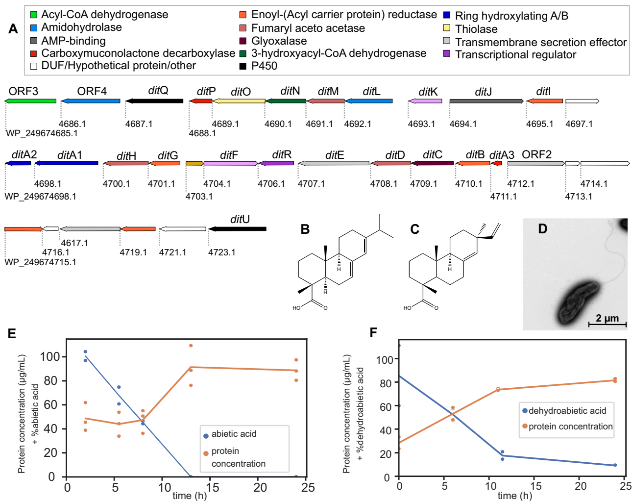
Fig. 4 | The genetic organization of the Pseudomonas abietivorans dit cluster and growth on resin acids.
