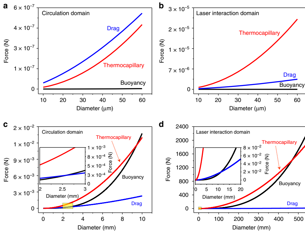
Fig. 4 Force analysis. a, b Comparison of drag force, buoyant force and thermocapillary force at the circulation domain ( a ) and the laser interaction domain ( b ) for the pore size range studied in this work. c, d Forces as a function of pore diameter. The critical pore size for buoyant force to overcome drag force is 2.5 mm at the circulation domain ( c ) and 11 mm at the laser interaction domain ( d ), which are even larger than the size of a typical melt pool in the LPBF process. The critical pore size for buoyant force to be larger than the thermocapillary force is even larger, 9.5 mm at the circulation domain ( c ) and 470 mm at the laser interaction domain ( d ). The inset (in c and d ) corresponds to the area marked by the yellow rectangle
