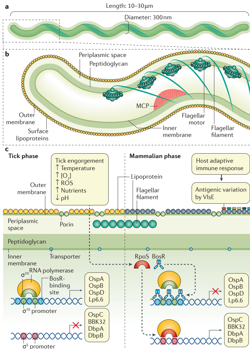
Figure 3 | Morphology and cellular architecture of Borrelia burgdorferi . a | Borrelia burgdorferi has a flat-wave morphology, is ~300 nm in diameter and 10–30 \mu m in length. b | A coloured model of one end of B. burgdorferi . The flagellar filaments are confined to the periplasmic space and are anchored to each cell pole by the flagellar motors, which are located next to methyl-accepting chemotaxis proteins (MCPs) that direct movement. c | The outer membrane of B. burgdorferi consists of a lipid bilayer that is heavily decorated with lipoproteins. Different sets of lipoproteins are expressed on the surface in the tick or mammalian environments. When a larval tick acquires B. burgdorferi from an infected mammalian host, the bacteria express tick-phase lipoproteins in the tick midgut. After larval ticks moult to nymphal-stage ticks and when these ticks feed, cues from tick engorgement block the expression of tick-phase lipoproteins and activate the expression of mammalian-phase lipoproteins through a complex regulatory network, including but not limited to Borrelia oxidative stress regulator (BosR) and the RNA polymerase alternative \sigma -factor RpoS. As the host mounts an adaptive immune response to B. burgdorferi , outer-surface protein C (OspC) is downregulated and VlsE, a lipoprotein that undergoes antigenic variation, is upregulated and expressed on the bacterial surface. The regulatory network for the adaptation of B. burgdorferi to different environments is much more complex than depicted in this figure; for example, the pathways leading to the activation of BosR and RpoS are still being determined, RpoS-dependent expression of lipoproteins could involve mechanisms other than the recruitment of RNA polymerase, the expression of some mammalian-phase-specific lipoproteins, such as VlsE and complement regulator-acquiring surface proteins (CRASPs), is not regulated through RpoS and not all tick-phase-specific lipoproteins are directly repressed by BosR. Lp6.6, 6.6-kDa lipoprotein; ROS, reactive oxygen species.
