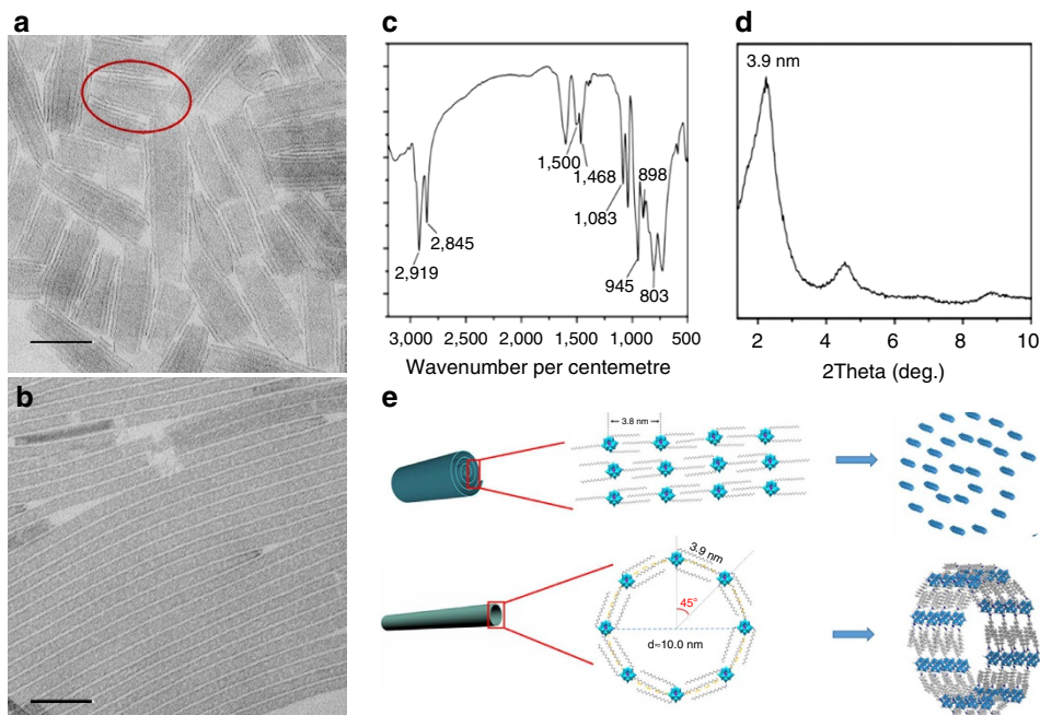
Figure 7 | POM SWNTs. Increasing the temperature or elongating the reaction time would convert the POM nanorolls (a) to SWNTs (b). Scale bar, 50 nm. The roll in the red circle shows an unequal number of ridges, indicating that it is indeed a roll but not a multi-wall tube. In the FT-infrared data, the peaks at 803\text{ cm}^{-1} and 898\text{ cm}^{-1} are assigned to the O–W–O antisymmetric stretching vibration modes of the bridging oxygen. The peak at 945\text{ cm}^{-1} corresponds to the \text{W}=\text{O} stretching mode of terminal oxygen. The peak at 1,083\text{ cm}^{-1} is ascribed to the P–O stretching mode. The peaks at 2,919\text{ cm}^{-1} and 2,845\text{ cm}^{-1} correspond to the \text{CH}_2 and \text{CH}_3 stretching vibrations and the peaks at 1,500 and 1,468\text{ cm}^{-1} correspond to the N–H mode, suggesting that the amine in the precursor exists in SWNTs. (d) SAXRD of POM nanotubes indicates a periodic distance of 3.9 nm. The infrared and SAXRD spectra of nanorolls show similar results to the nanotubes. Taking all these results into account, the structures of the nanorolls and SWNTs are depicted in (e). The cross-sectional perimeter of the nanotubes is \pi d , and when it is divided by the distance between two clusters (that is, 3.9 nm), we determine that first eight POM clusters form a ring, and these rings further self-assemble into nanotubes.
