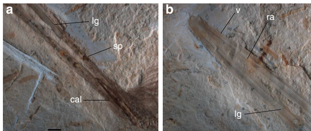
Figure 2 | Details of tail feather of specimen UFRJ-DG 031 Av. (a) Proximal end. (b) Distal end. cal, calamus; lg, longitudinal groove; ra, rachis; sp, colour spot; v, vane. Scale bar, 2.5 mm.
