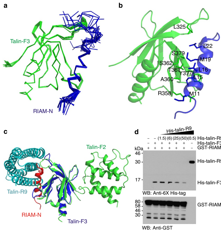
Figure 3 | Structure of RIAM-N/talin-F3 complex reveals a mechanism for talin unmasking. (a) Superposition of 20 calculated RIAM-N/talin-F3 complex structures with lowest energies, showing a well-defined structure. (b) Cartoon representation of the structure with the lowest energy. The side chains of the residues involved in the intermolecular interaction are displayed to demonstrate the hydrophobic interface. (c) The structure of talin-F3 (blue) bound to RIAM-N (red) was superimposed onto the talin-F2F3 (green) bound to talin-R9 (cyan), showing that RIAM-N sterically interferes with the autoinhibitory interface. (d) Pull-down assay to show that RIAM-1-306 competes with talin-R9 for binding to talin-F3. With increasing amounts ( \mu\text{g} ) of talin-R9, the population of RIAM-bound talin-F3 is reduced as visualized by the western blot analysis with anti-His (top panel). Western blot analysis of the bound GST-RIAM-1-306 with anti-GST is used as a control (bottom panel).
