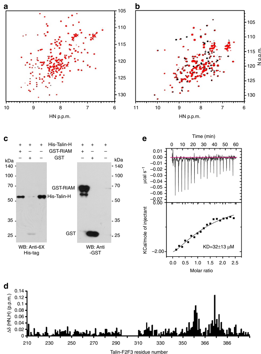
Figure 2 | RIAM interaction with talin-F3. (a) 2D 1 H- 15 N HSQC spectra of 40 μM 15 N-talin-F0F1 in the absence (black) and presence of 80 μM RIAM-1-306 (red). (b) 2D 1 H- 15 N HSQC spectra of 40 μM 15 N/ 2 H-talin-F2F3 in the absence (black) and presence of 80 μM RIAM-1-306 (red). (c) Pull-down assay to show that GST-RIAM-1-306, but not GST control, binds to talin-H. (d) Chemical shift change profile of talin-F2F3 by RIAM-1-306, showing that talin-F3 is specifically perturbed by RIAM-1-306. (e) K_D between talin-F2F3 and RIAM-1-306 by ITC.
