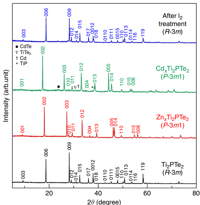
Figure 2 | X-ray diffraction patterns of Ti_2PTE_2 and (de)intercalated materials. From bottom to top: Ti_2PTE_2 , Zn_xTi_2PTE_2 ( 300^\circ C , 48 h, p = 0.4 ), Cd_xTi_2PTE_2 ( 200^\circ C , 48 h, p = 0.4 ), deintercalated product after I_2 treatment of Zn_xTi_2PTE_2 at room temperature. Peaks with symbols show tiny amount of impurity phases (CdTe, TiTe_2 and so on) for Cd intercalation.
