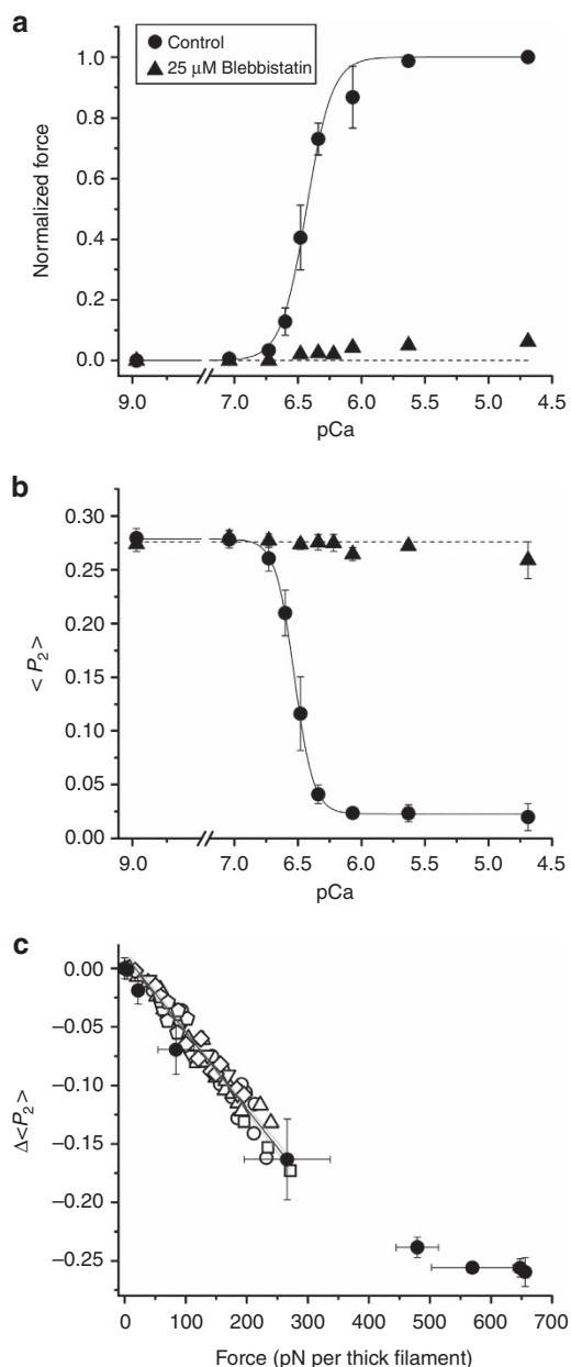
Figure 5 | RLC orientation change during active isometric contraction. (a) Steady force at different pCa normalized by the maximum force at pCa 4.7 ( 267 \pm 10 kPa; mean \pm s.e., n = 5 fibres) in the presence (triangles; mean \pm s.e., n = 5 fibres; error bars are smaller than symbol size) and absence (circles; mean \pm s.e., n = 5 fibres) of 25 \mu M Blebbistatin. Sarcomere length 2.40 \mu m, 25 ^{\circ} C, 5% Dextran. (b) \langle P_2 \rangle for the E-helix probe in the same experiments. (c) Force-dependence of \Delta \langle P_2 \rangle during active contraction (filled circles, from a,b) compared with that for the end of phase 2 after force steps in the presence of 25 \mu M Blebbistatin (data from Fig. 4b).
