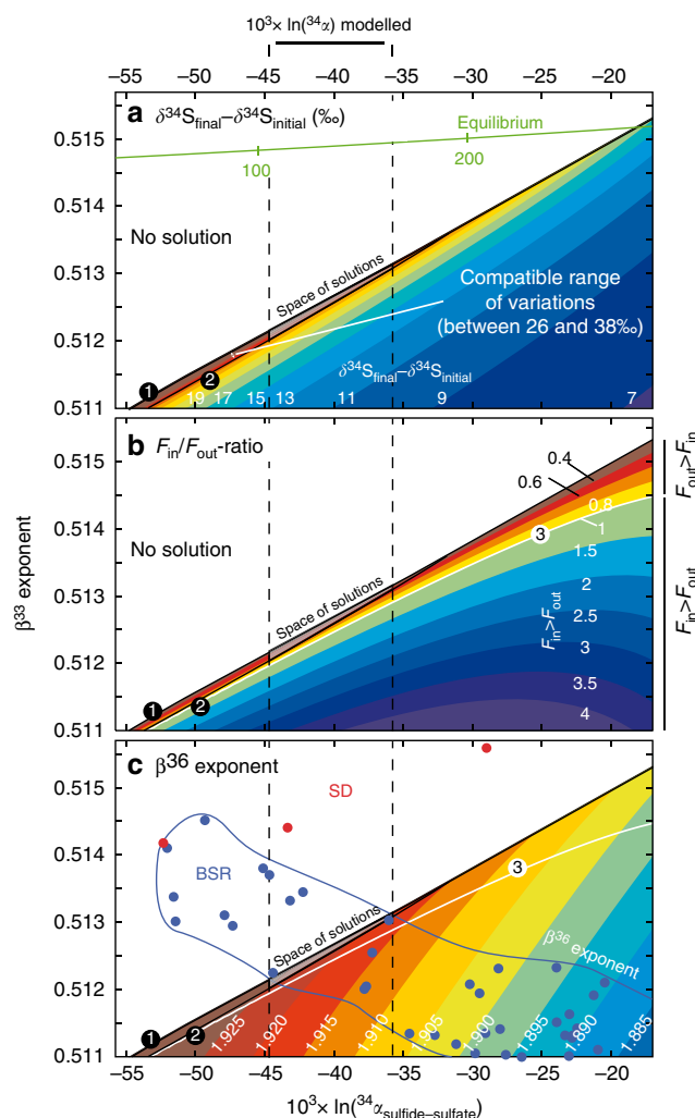
Figure 3 | Model results in three 1,000\ln(^{34}\alpha) versus ^{33}\beta – exponents diagrams. The results show the combinations of ^{33}\beta , ^{34}\alpha and F_{in}/F_{out} that fit our data in 1,000\ln(^{34}\alpha) versus ^{33}\beta – exponents diagrams. (a) illustrates the \delta^{34}\text{S}_{\text{CAS}} -range (that is, \delta^{34}\text{S}_{\text{CASfinal}} - \delta^{34}\text{S}_{\text{CASinitial}} ) compatible with our data. The curve #2 delimitates the field below which the difference between \delta^{34}\text{S}_{\text{CASfinal}} and \delta^{34}\text{S}_{\text{CASinitial}} values ( +38\text{‰} and +12\text{‰} , respectively) is too low (that is, \delta^{34}\text{S}_{\text{CASfinal}} - \delta^{34}\text{S}_{\text{CASinitial}} < 26\text{‰} ) to account for the high \delta^{34}\text{S}_{\text{CAS}} -values measured in our section. (b) illustrates the F_{in}/F_{out} -ratios that fit the observed \delta^{34}\text{S}_{\text{CAS}} versus \Delta^{33}\text{S}_{\text{CAS}} slope for each pair of ^{33}\beta , ^{34}\alpha . The white curve #3 highlights the steady-state conditions, where F_{in} = F_{out} . (c) represents the combinations of ^{33}\beta and ^{34}\alpha compatible with our data for different ^{36}\beta values. The intercept between the modelled space of solution and results from BSR experiments allows restricting further the space of solution. The grey polygon represents the final solution space.
