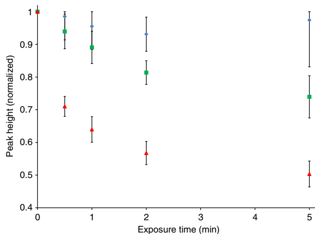
Figure 5 | Methylene blue signal degradation by prolonged laser exposure. Normalized heights of the 447 \text{ cm}^{-1} Raman mode of Ag-MB gathered at 373 \text{ K} and in inert \text{N}_2 atmosphere after exposure to no laser (control, blue diamonds), 532-nm laser (green squares) or 785-nm laser (red triangles) for a given periods of time. The 785-nm laser shows significant signal degradation enhancement compared with the 532 nm and control samples.
