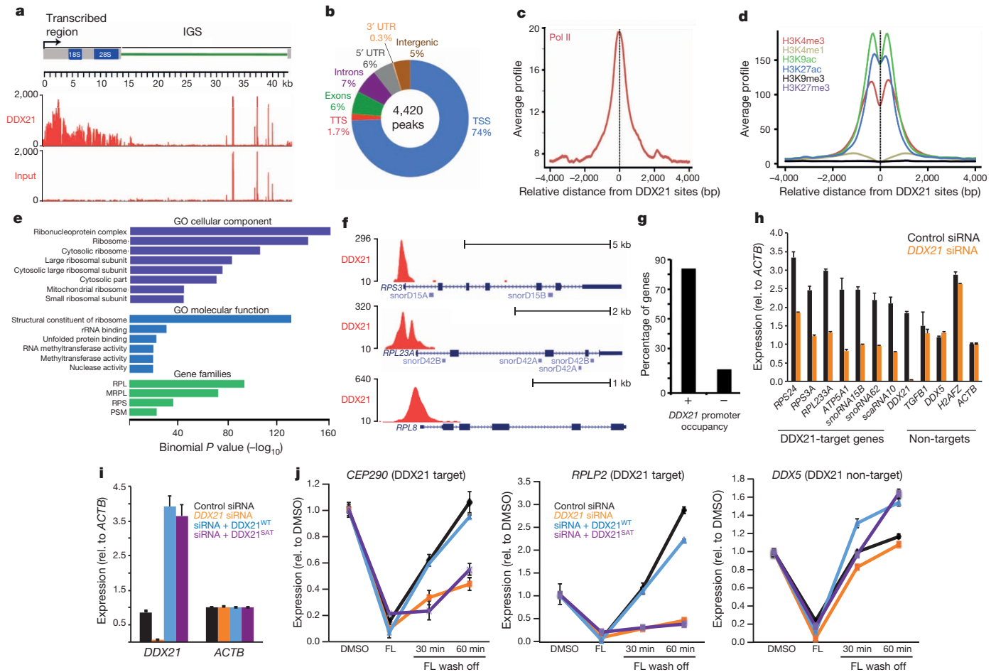
Figure 1 | DDX21 associates with actively transcribed ribosomal genes.
