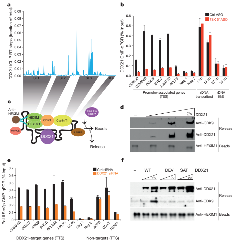
Figure 4 | DDX21 promotes release of P-TEFb from the 7SK snRNP. a , DDX21 WT iCLIP reads mapped to the 7SK snRNA. The four stem-loops (SL1–4) are marked below the iCLIP reads and are shadowed on the cartoon in c . b , ChIP-qPCR of DDX21 in control or 5'-7SK-antisense oligonucleotide (ASO)-treated HEK293 cells at representative Pol II-regulated, DDX21-target gene promoters, negative control regions (Neg), and the rDNA locus. Data are mean and s.d. For DDX21-target genes the difference between control ASO and 5' ASO is significant at P < 0.05 (Student's t -test). c , d , Schematic (left) and western blot analysis (right) of a P-TEFb release assay as a function of increasing amounts of DDX21 WT . e , ChIP-qPCR of Pol II Ser2p of representative Pol II-regulated genes at their transcriptional termination sites (TTS) in control or DDX21-siRNA-treated cells. Data are mean and s.d. of three independent experiments. f , Western blot analyses of a P-TEFb release assay with either DDX21 WT or catalytically impaired DDX21 DEV and DDX21 SAT .
