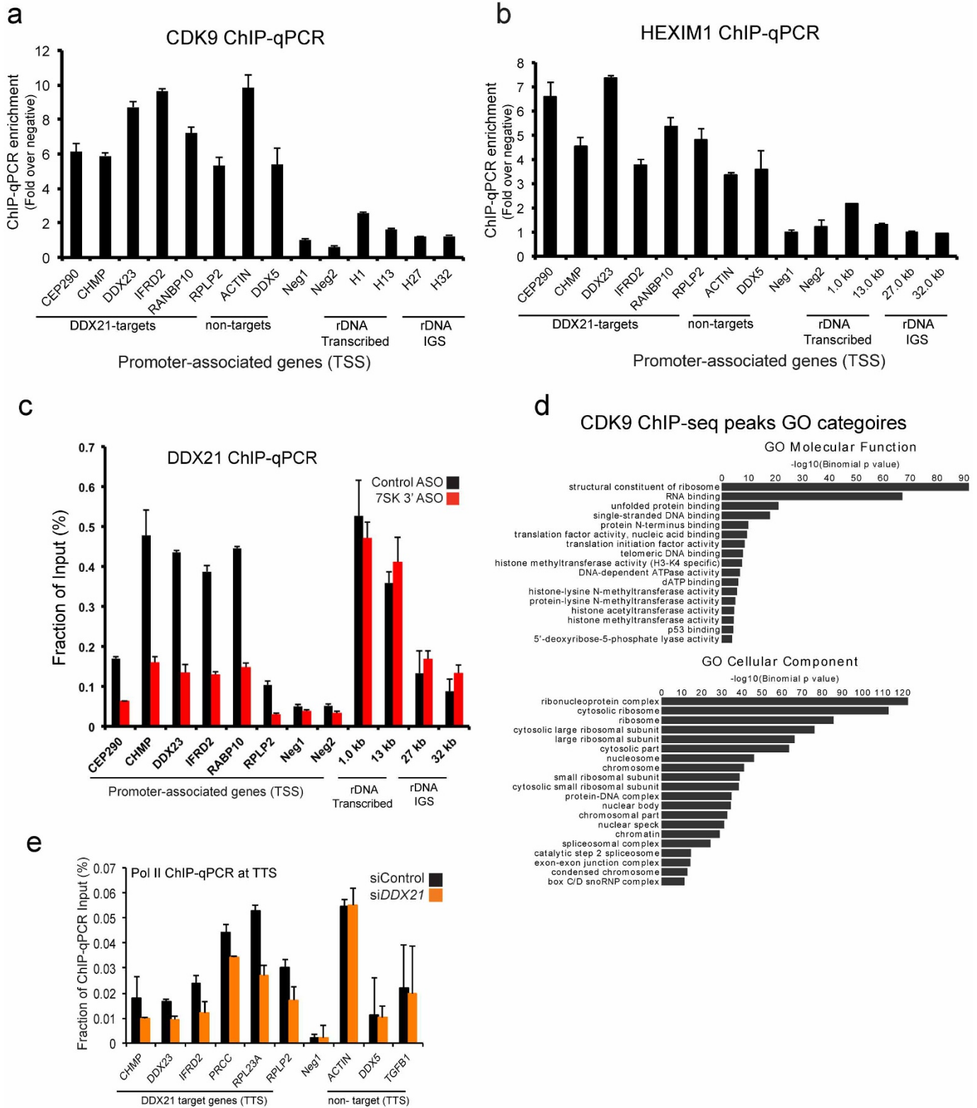
Extended Data Figure 9 | Binding of the DDX21-7SK snRNP at ribosomal gene promoters. a , b , ChIP-qPCR of CDK9 ( a ) and HEXIM1 ( b ) in HEK293 cells at representative Pol II-regulated, DDX21-target and -non-target gene promoters, negative control regions, and the rDNA locus. c , ChIP-qPCR of DDX21 in control or 3'-7SK-ASO-treated HEK293 cells at representative Pol II-regulated, DDX21-target gene promoters, negative control regions, and the rDNA locus. For the promoter-associated genes, P \leq 0.05 (Student's t -test)
