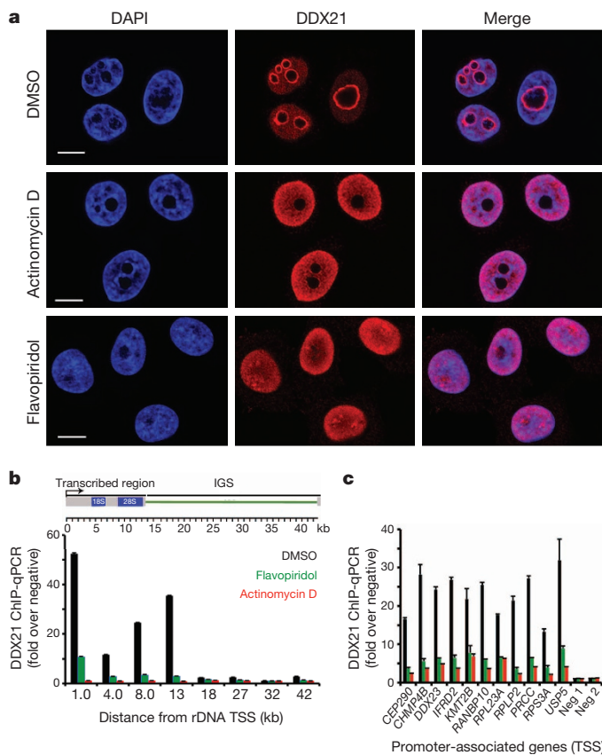
Figure 2 | DDX21 chromatin association is sensitive to Pol I and Pol II transcriptional status. a , Representative immunofluorescence images of methanol-fixed HEK293 cells after 1-h incubation with DMSO, actinomycin-D (50 ng ml -1 ) or flavopiridol (1 μM). Scale bars, 10 μm. DAPI, 4',6-diamidino-2-phenylindole. b , c , ChIP-qPCR analysis in HEK293 cells sampling DDX21 genomic occupancy at the rDNA locus and at a representative panel of Pol II-regulated, DDX21-target promoters, upon treatment with DMSO, actinomycin-D or flavopiridol. Data are mean and s.d. of three independent experiments. Neg, negative controls.
