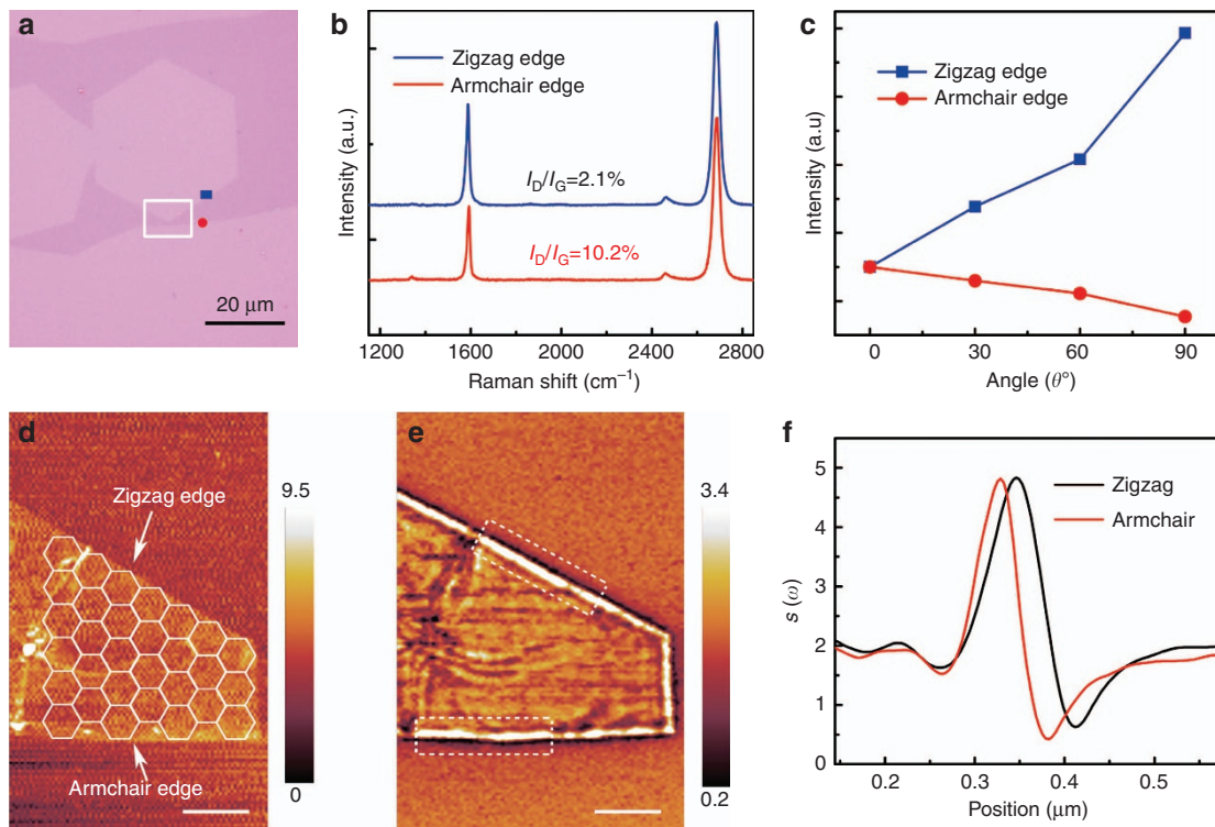
Figure 5 Effect of edge chirality on graphene plasmon. (a) Optical image, scale bar = 20\ \mu\text{m} . (b) Typical Raman spectra measured at the zigzag edge and armchair edge (inner and outer edges). (c) Polarization dependence of the G peaks of the zigzag edge and armchair edge indicated by blue square and red circle in a. (d) AFM topography of a graphene ribbon with controlled edges (indicated by white arrows). (e) Near-field optical amplitude, obtained simultaneously with the AFM topography shown in d, at an infrared wavelength of \lambda_0 = 11.086\ \mu\text{m} . Scale bar = 500\ \text{nm} . (f) Experimental s(\omega) line profiles obtained by averaging 20 such profiles in the region (white dashed rectangles in e) at edges with different chirality (zigzag or armchair), revealing a broader plasmon at the zigzag edge.
