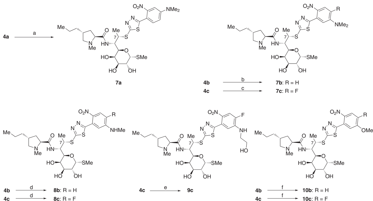
Scheme 2 Synthesis of (7 S )-7-(5-phenyl-1,3,4-thiadiazol-2-yl-thio)-7-deoxylincomycin derivatives. Reagents: (a) 2 M dimethylamine in methanol, 80 °C, 16 h, 81%; (b) 2 M dimethylamine in methanol, rt, 1 h, 87%; (c) 2 M dimethylamine in methanol, 50 °C, 3.5 h, 87%; (d) 40% methylamine in methanol, rt, 1 h, 75% from 4b to 8b , 98% from 4c to 8c ; (e) 2-aminoethanol, 50 °C, 2 h, 86%; (f) 28% sodium methoxide methanol solution, rt, 64% from 4b to 10b , 70% from 4c to 10c .
