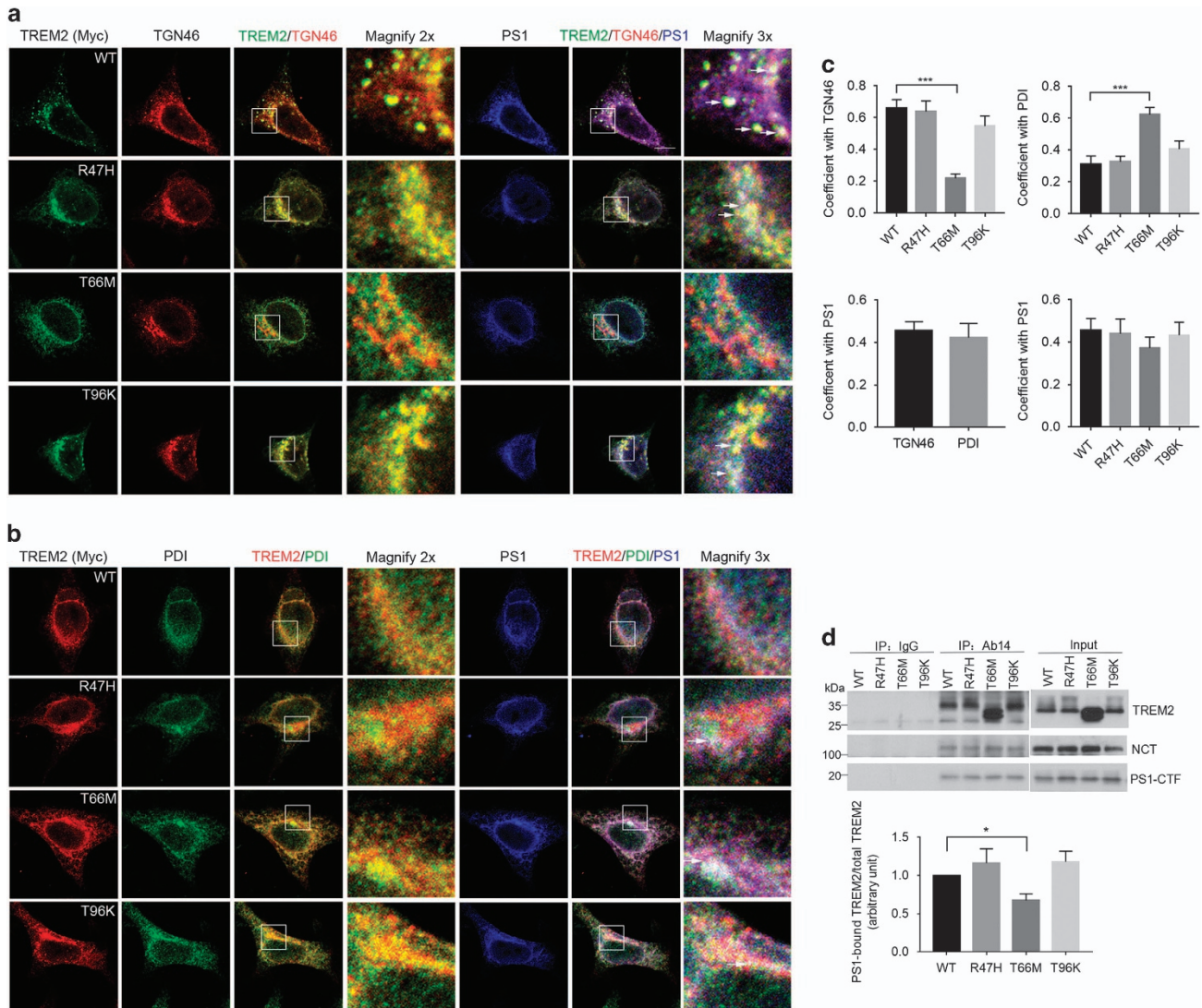
Figure 2 Mutations in TREM2 affect colocalization and interactions between TREM2 and presenilin 1 (PS1). PS1 was transfected into HEK293 cells stably expressing Myc-tagged TREM2 WT or TREM2 mutants as indicated. (a, b) Cells were then subjected to immunostaining with antibodies against Myc, PS1, and TGN46 (a marker for the Golgi, a) or PDI (a marker for the ER, b). White arrows in magnified images indicate colocalizing overlap for TREM2, PS1 and TGN46/PDI. Scale bars for a, b, 10 \mu m. (c) Quantification of colocalized signals. Pearson's correlation coefficient is shown. *** P < 0.001 , n = 3 independent experiments, one-way ANOVA with Dunnett's post hoc analysis. (d) Cell lysates were immunoprecipitated with the PS1 antibody Ab14 or normal IgG. TREM2, NCT and PS1-CTF were detected by immunoblotting. The levels of precipitated TREM2 WT and mutants were normalized to the input. * P < 0.05 , n = 3 , Student's t -test.
