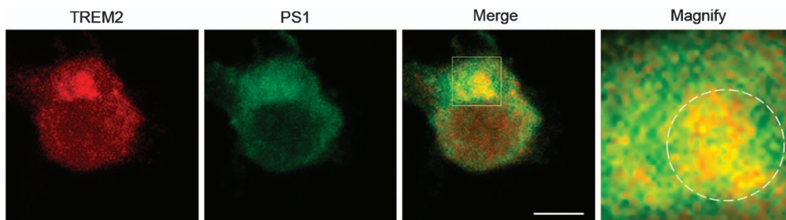
Figure 3 Endogenous TREM2 partially colocalizes with endogenous presenilin 1 (PS1) in microglial BV2 cells. BV2 cells were immunostained with antibodies against PS1 and mouse TREM2. White circles in magnified images indicate some colocalizing overlap between TREM2 and PS1 in Golgi-like structures. Scale bar, 5 \mu m.
