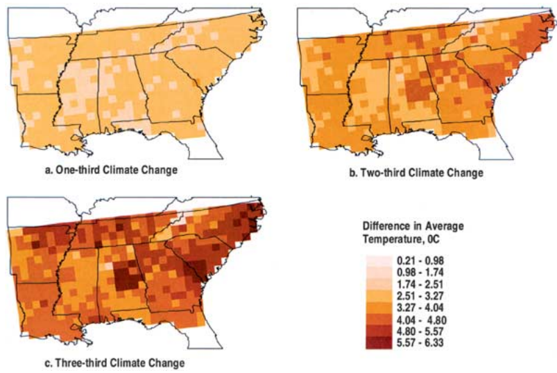
Figure 2. Change in temperature ( ^{\circ}\text{C} ) relative to 1960–1995 baseline climate simulated by the RegCM model. (a) 1/3 of 2 \times \text{CO}_2 climate. (b) 2/3 of 2 \times \text{CO}_2 climate. (c) 3/3 of 2 \times \text{CO}_2 climate (or ‘equivalent doubling \text{CO}_2 equilibrium’).
