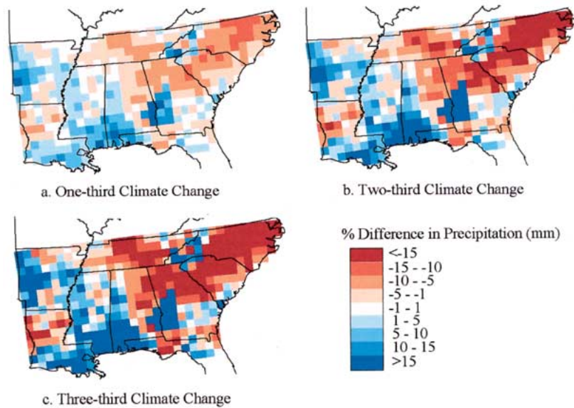
Figure 3. Change in precipitation (%) relative to 1960–1995 baseline climate simulated by the RegCM model. (a) 1/3 of 2 \times \text{CO}_2 climate. (b) 2/3 of 2 \times \text{CO}_2 climate. (c) 3/3 of 2 \times \text{CO}_2 climate (or ‘equivalent doubling \text{CO}_2 equilibrium’).
