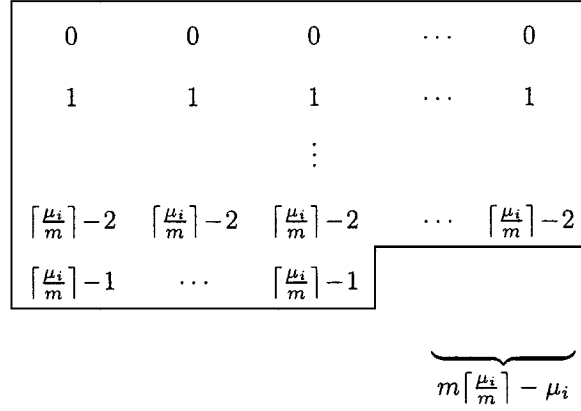
Figure 5. First \mu_i elements of the sequence \langle 0 \rangle^m \langle 1 \rangle^m \langle 2 \rangle^m \dots
