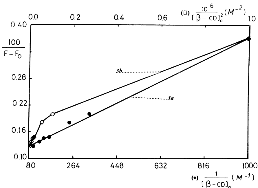
Figure 3. Double reciprocal plots for compound 4. (a) A linear relationship is established when the data are plotted assuming a 1 : 1 NBD : β-CD stoichiometry (Equation 2). (b) A downward concave curvature is observed when the data are plotted assuming a 1 : 2 stoichiometry (Equation 3).
