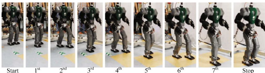
Fig. 8 Snapshots of walking forward with step length 0.2 m and stabilizer module on.
