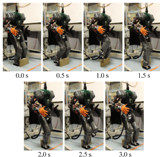
Fig. 10 Snapshots of successful stepping over a large obstacle.
