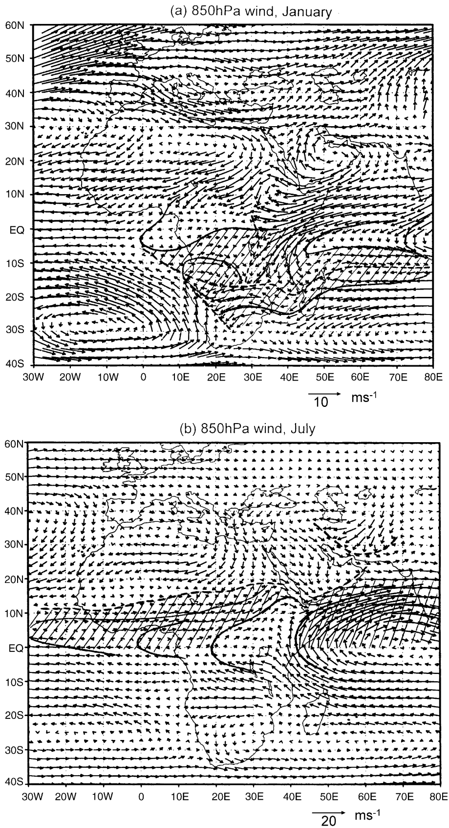
Fig. 2. Climatologically mean 850 hPa winds ( \text{ms}^{-1} ) for the African continent in (a) January and (b) July based on the NCEP/NCAR reanalysis data from 1950 to 1999. Shaded areas denote the domain influenced by the cross-equatorial flows. The solid lines are streamlines and the dashed lines indicate the ITCZ.
