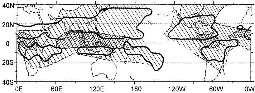
Fig. 9. Global monsoon distributions summarized based on the analysis of cross-equatorial flow reversals and dry/wet spell transition. Three cross-hatched areas near the Equator denote the annual-mean BT < 244 K. Six regions in the subtropics are affected by the dry/wet spell transition. The single-hatched areas represent the regions influenced by cross-equatorial flows
