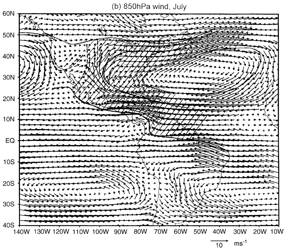
Fig. 5. Same as in Fig. 2 but for the South and North American continents. Dashed lines in the central North America indicate the convergence and divergence axes
