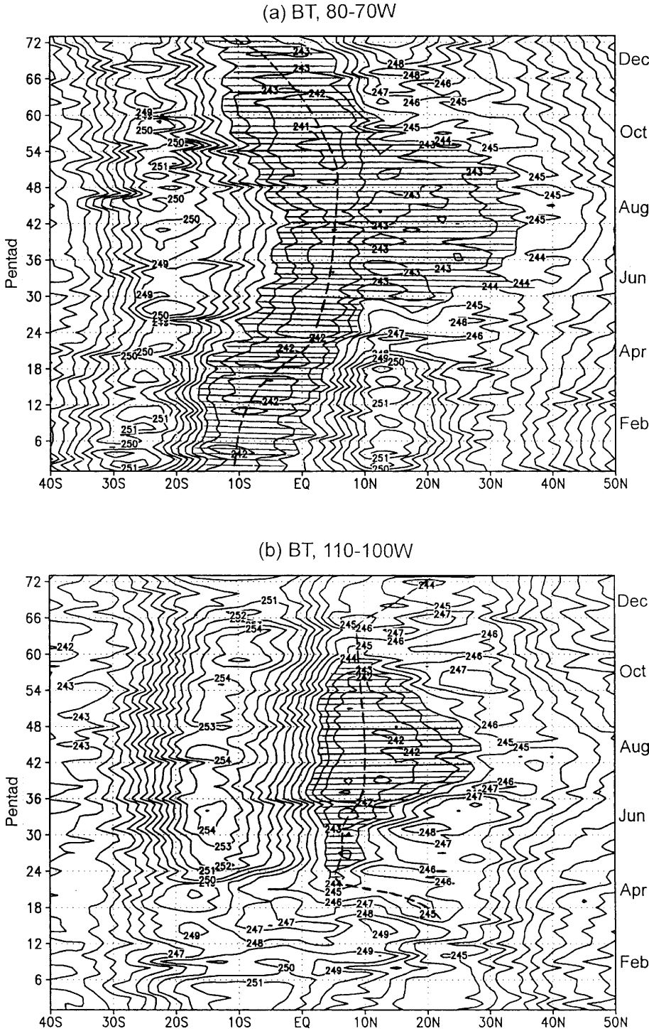
Fig. 6. Same as in Fig. 3 but for (a) 80–70° W and (b) 110–100° W
