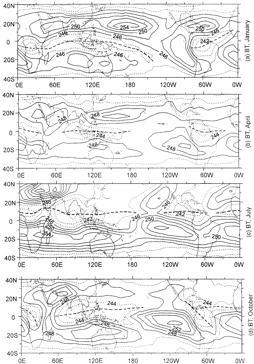
Fig. 1. Climatology of global BT (K) for (a) January, (b) April, (c) July, and (d) October based on the HIRS12 data from 1980 to 1995. Lightly dashed areas outline BT < 244 K. Heavily dashed lines indicate the wet maximum or deep convective zone
