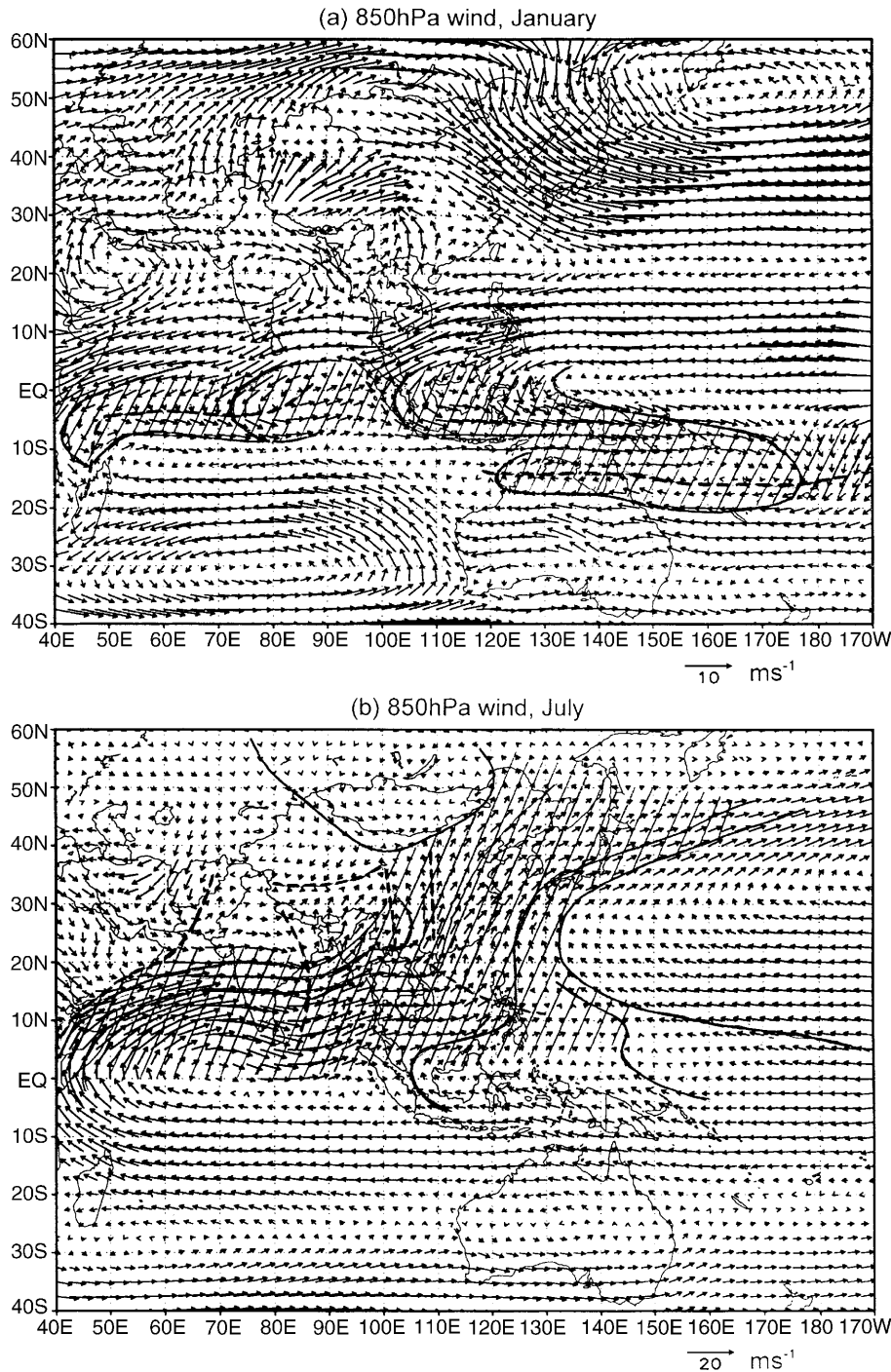
Fig. 7. Same as in Fig. 2 but for the Asian–Australian region. Dashed lines in central China indicate the convergence and divergence axes
