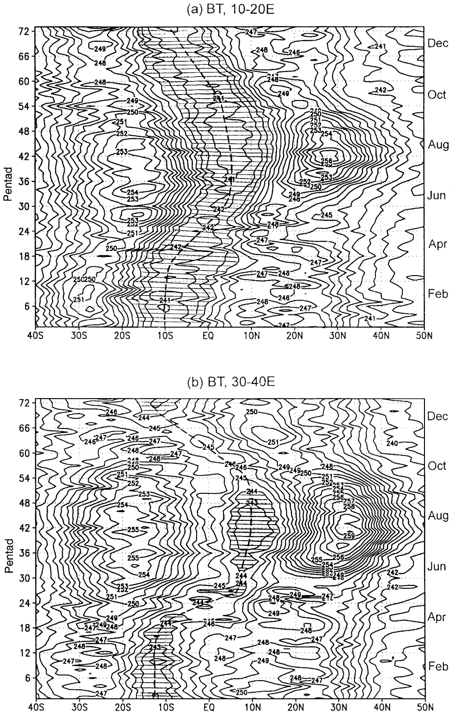
Fig. 3. Time-latitude section of climatological pentad-mean BT (K) along (a) 10–20° E and (b) 30–40° E based on the HIRS12 data from 1980 to 1995. Shaded areas denote the BT lower than 244 K and dashed lines the maximum of BT
