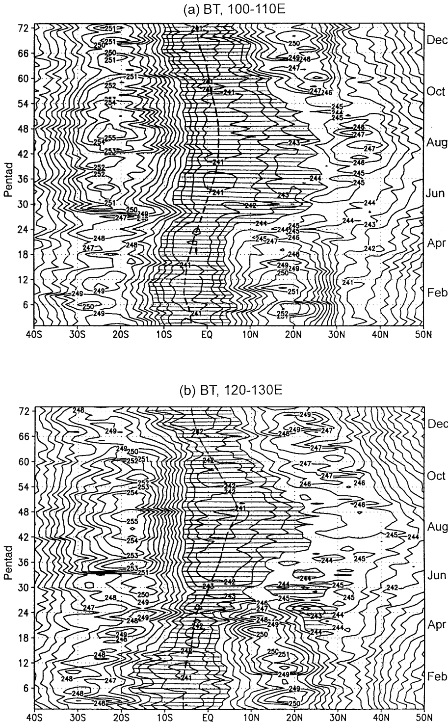
Fig. 8. Same as in Fig. 3 but for (a) 100–110° E and (b) 120–130° E
