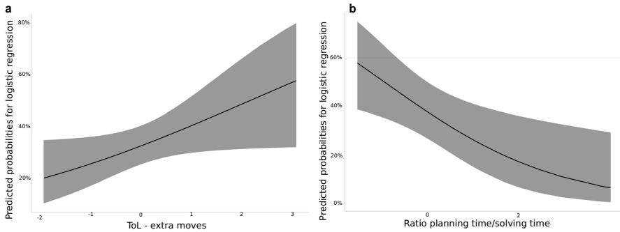
Fig. 1 (a) Predicted probabilities for a binomial logistic model using the ggpredict function, that predicts values for all possible levels and values from a model's predictors. Predictor variable: EM ToL (z-scores). Outcome variable: Sexual intercourse before 15 years old. (b) Predicted probabilities for a binomial logistic regression model using the ggpredict function. Predictor variable: Ratio planning time/solving time (RPT/ST) for all trials in ToL (z-scores). Outcome variable: Sexual intercourse before 15 years old. The shaded area represents the 95% confidence bands
