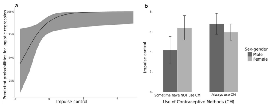
Fig. 2 (a) Predicted probabilities for a binomial logistic model using the ggpredict function, that predicts values for all possible levels and values from a model's predictors. Predictor variable: IC_RT ToL (z-scores). Outcome variable: consistent use of CM. The shaded area represents the 95% confidence bands. (b) IC_RT by sex-gender and CM use. Error bars reflect \pm 2 standard error mean (SEM)
