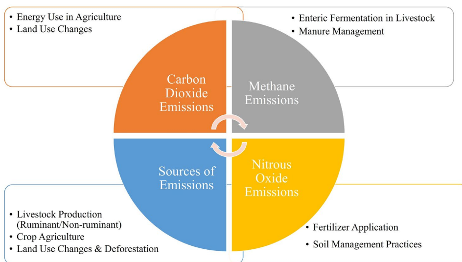
Fig. 2 Three primary GHG: CO 2 , CH 4 , and N 2 O, and their sources
