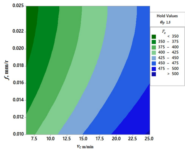
Fig. 16 Cutting force F_z vs f , and v_c
