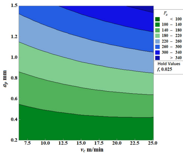
Fig. 8 Cutting force F_z vs a_p and v_c [40]
