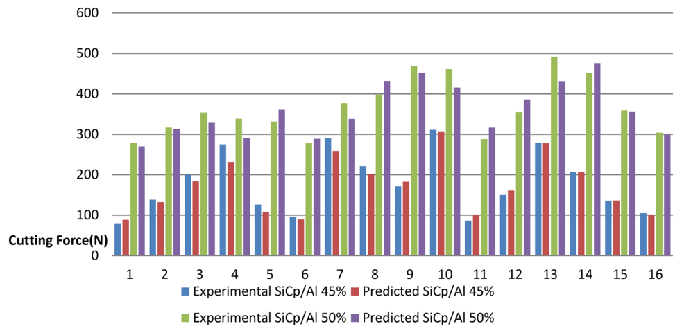
Fig. 25 Comparisons of Experiment values and Predicted values of Cutting force of F_z of SiCp/Al 45% and 50%
