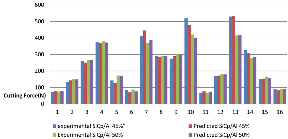
Fig. 24 Comparisons of Experiment values and Predicted values of Cutting force of F_x , of SiCp/Al 45% and 50%
