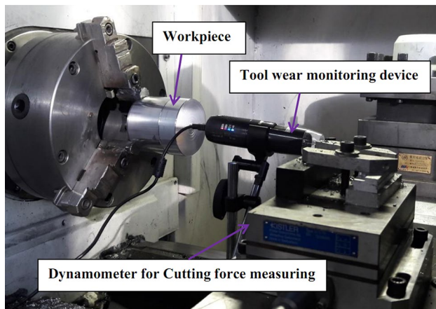
Fig. 1 Experimental setup
