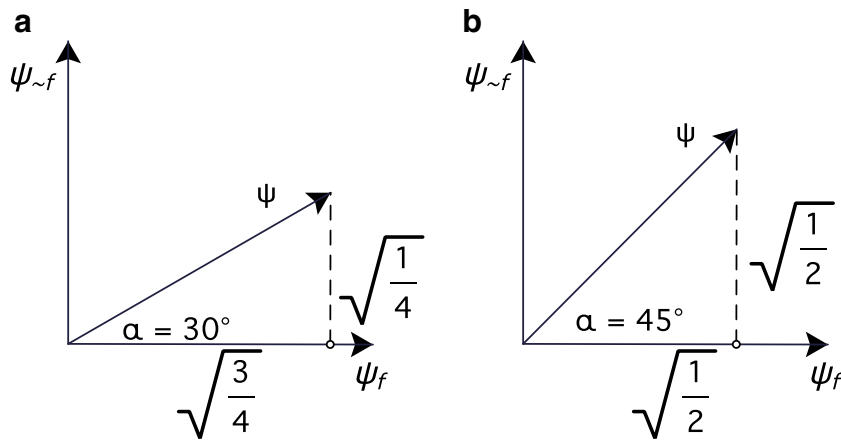
Fig. 1 a An initial knowledge state vector for “Is Linda a feminist?” b A different initial knowledge state vector for “Is Linda a feminist”
