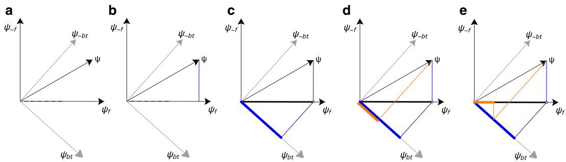
Fig. 2 a Setting up the two subspaces for the Linda problem with four basis vectors, where v is the initial state vector; b projecting the knowledge state vector onto the feminist basis vector; c projecting the resulting vector onto the bank teller basis vector; d projecting the knowledge state vector onto the bank teller basis vector; e projecting the resulting vector onto the feminist state vector
