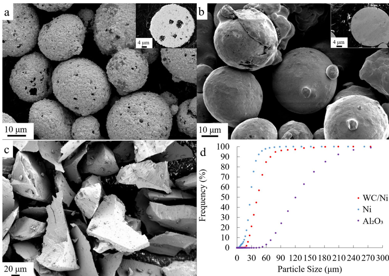
Fig. 2 Electron micrographs of the feedstock powders. a Composite WC/Ni powder. b Nickel powder. c Alumina erodent particles. d Particle size distribution of the WC/Ni, Ni, and \text{Al}_2\text{O}_3 powders
