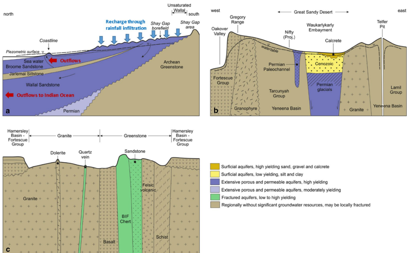
Fig. 7 Conceptual cross sections across a sandstone aquifers in the West Canning Basin, b Permian/Cenozoic paleochannels in the Paterson Province, and c typical BIF and fractured sandstones aquifers in the granite–greenstone terrain of the Pilbara region
