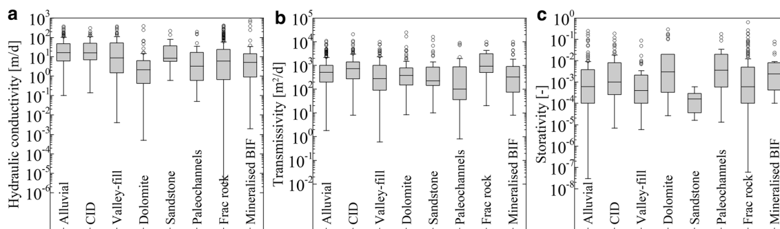
Fig. 8 Boxplots for the hydraulic properties collected for the aquifers identified in the Pilbara region. Alluvial coastal alluvial, CID channel iron deposit, Valley-fill , Dolomite karstified/weathered
