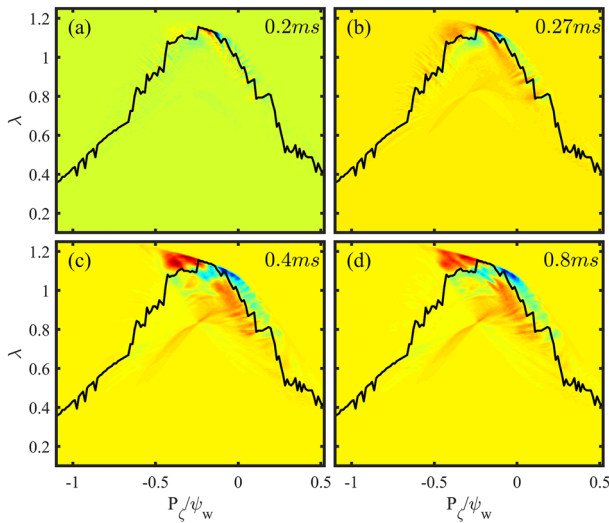
Fig. 8 Perturbed beam ion distribution function \delta f in (P_\zeta, \lambda) phase space at 0.2ms [panel (a)], 0.27ms [panel (b)], 0.4ms [panel (c)], and 0.8ms [panel (d)] from single mode ( n=4 ) simulation with zonal flows for a magnetic moment \mu B_a = 80\text{keV} . The black line represents the dominant resonance
