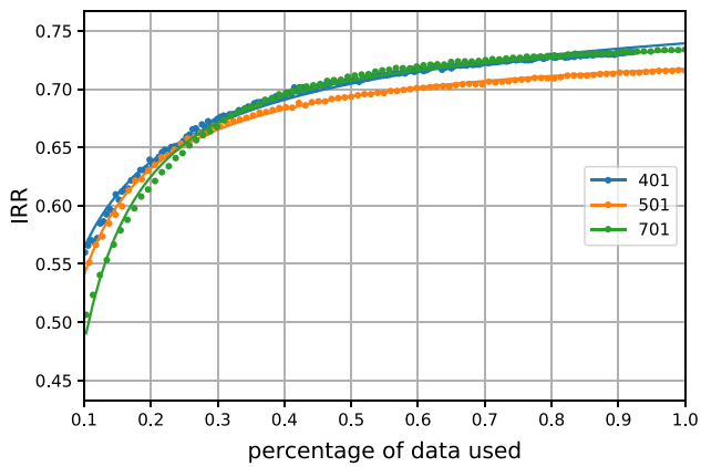
Fig. 6 Absolute Inter-Rater Reliability values, calculated using different percentage of data
