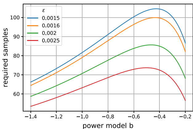
Fig. 8 Required sample size \eta (Eq. (26)) for a power model with given b to have the normalized derivation below a threshold \epsilon
