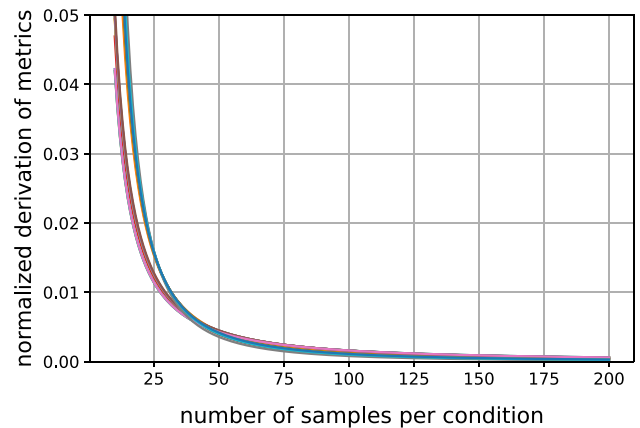
Fig. 7 Comparison of power models for the different CS datasets and all metrics (SRCC, RMS, CIW, EMD, IRR)
