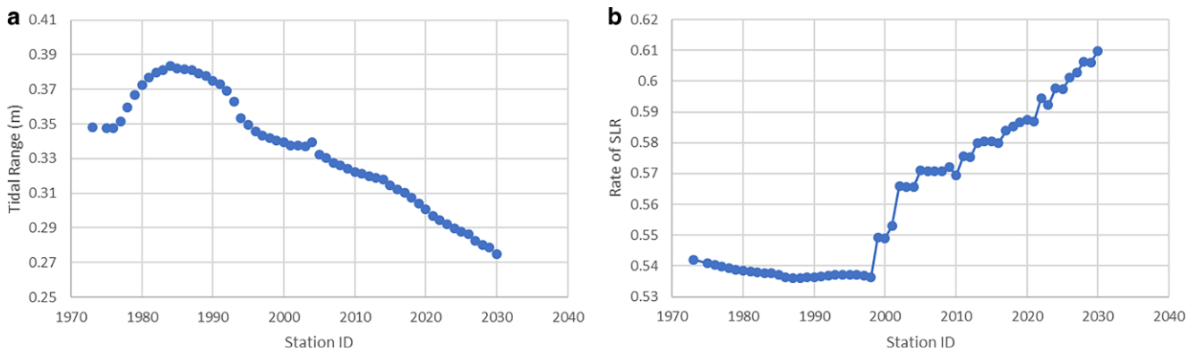
Fig. 6 a Average tidal range and b projected SLR rates according to the Copernicus model for 2041–2070 (Yan et al. 2020). Station IDs, plotted along the horizontal axis, indicate the specific locations for model calculations. Refer to Fig. 4 for a detailed map of these station locations
