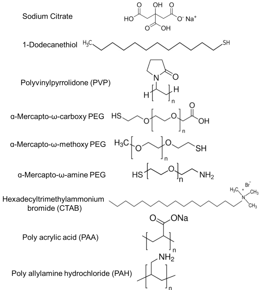
Fig. 3 Representative stabilizing ligand for plasmonic NPs
