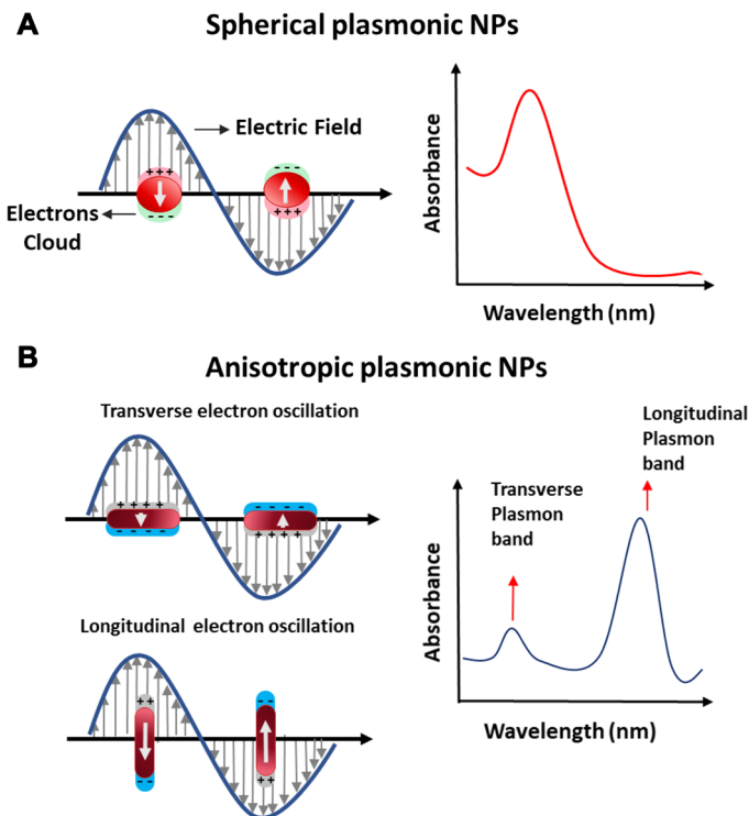
Fig. 1 Schematic representation of surface plasmon resonance (SPR) band in A spherical and B rod-shaped plasmonic nanoparticles (NPs)
