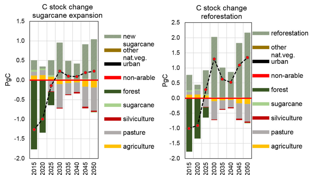
Fig. 9 Carbon change by land stock for sugarcane expansion and reforestation scenarios
