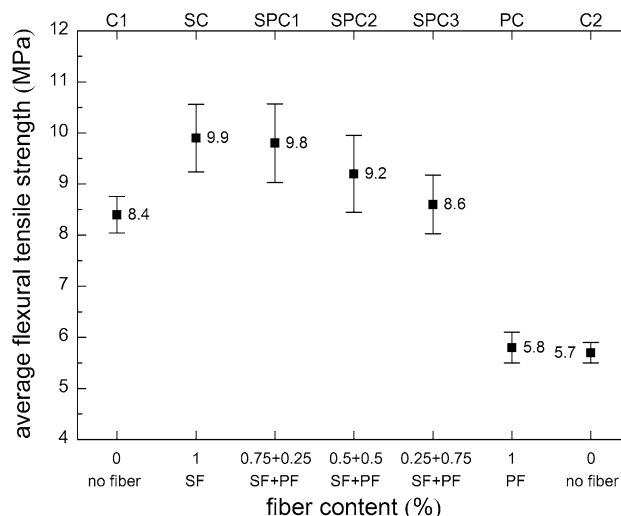
Fig. 5 Average flexural tensile strength
