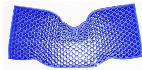
(d) Layers formed by buckled hexagonal infill
