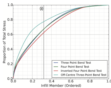
Fig. 17 Beam stress along potential lattice elements
