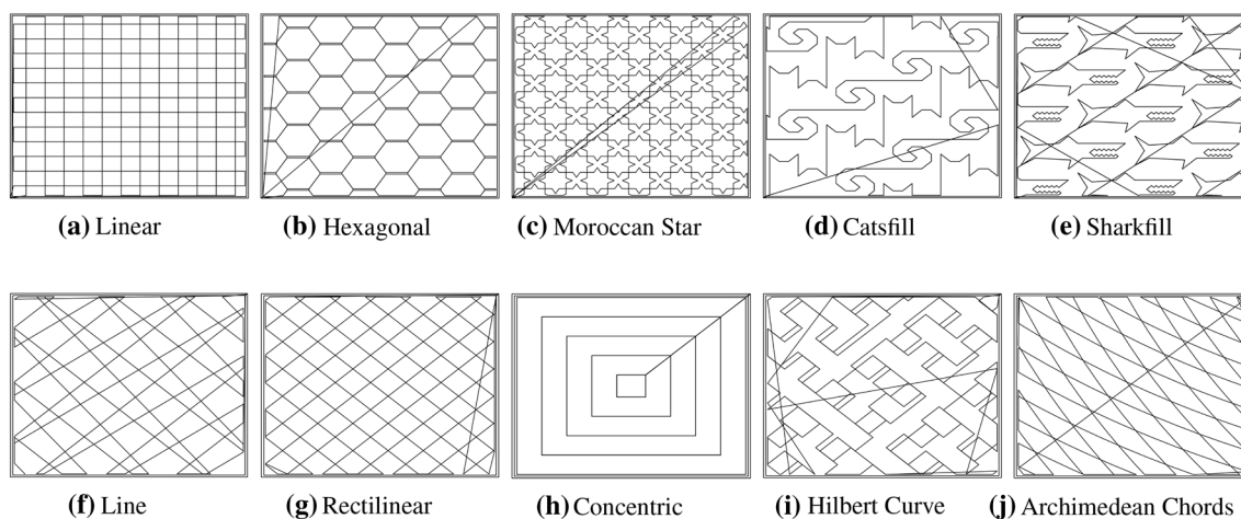
Fig. 1 Infill strategies from MakerWare (a–e) and Slic3r (f–j) software
